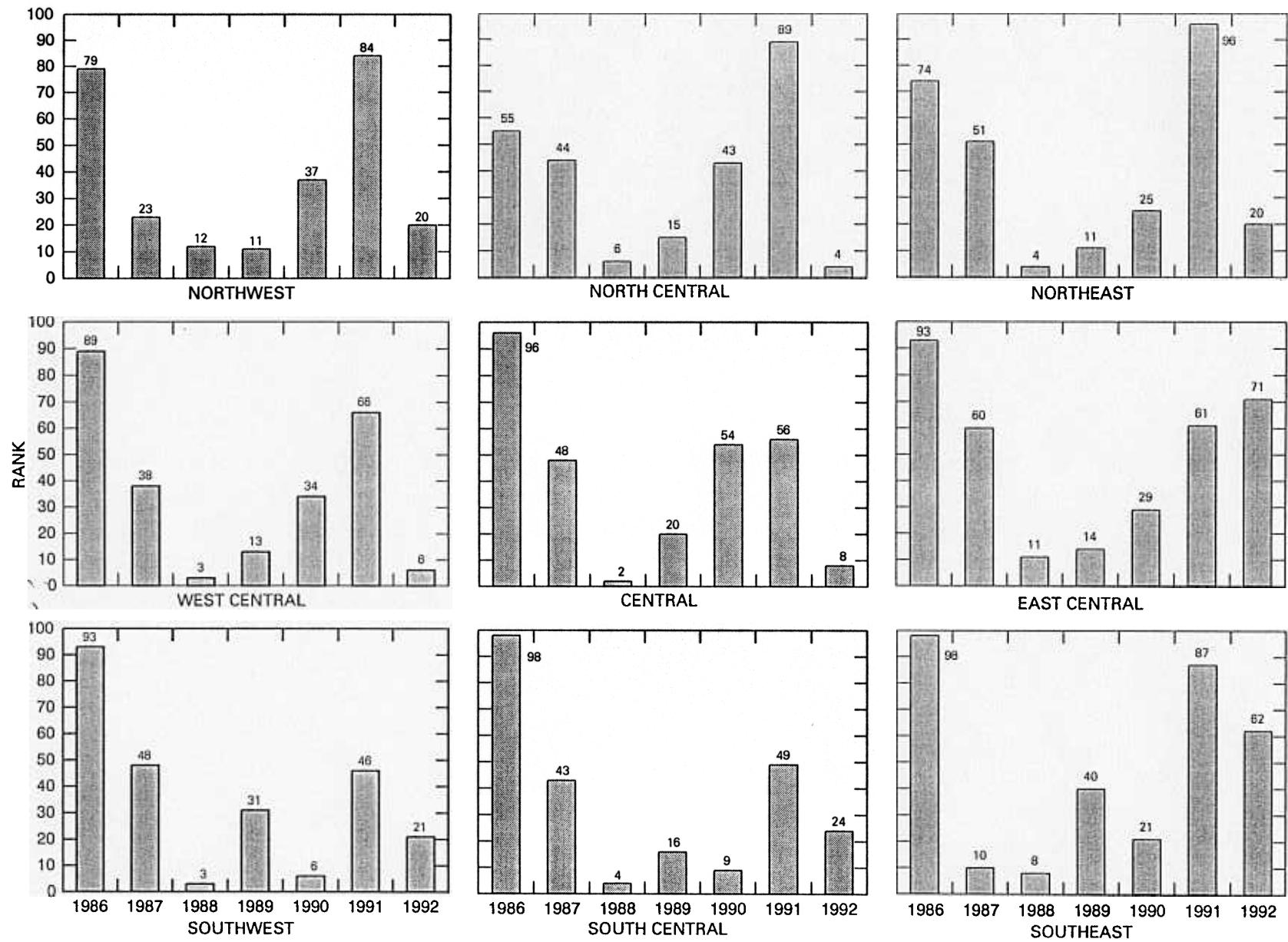
Figure 4. Rank of 1986-92 annual precipitation from 1895 through 1992 for each climatic division in North Dakota (1 indicates driest year, 98 indicates wettest year).
