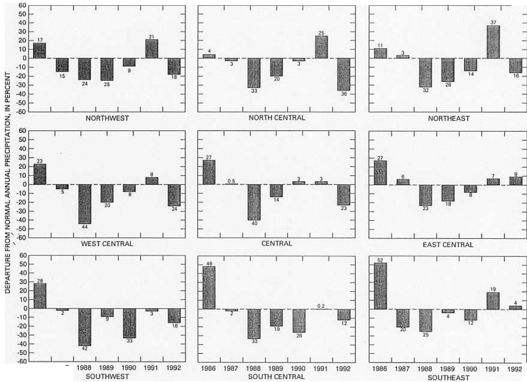
Figure 3. Departure from normal annual precipitation during 1986-92 for each climatic division in North Dakota.
