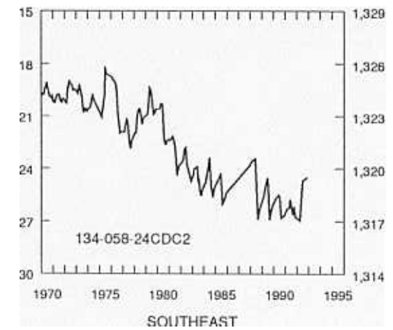
Figure 10. Ground-water levels in selected wells during 1970-92 for southwest and southeast climatic divisions in North Dakota.
