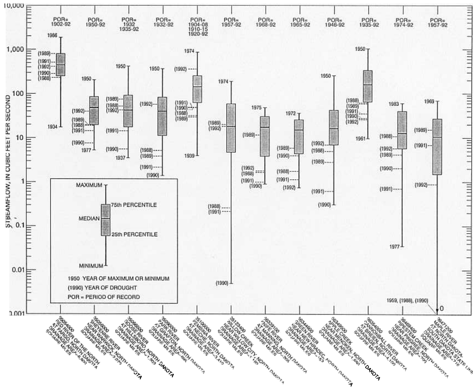
Figure 7. Streamflows at selected gaging stations in North Dakota.
