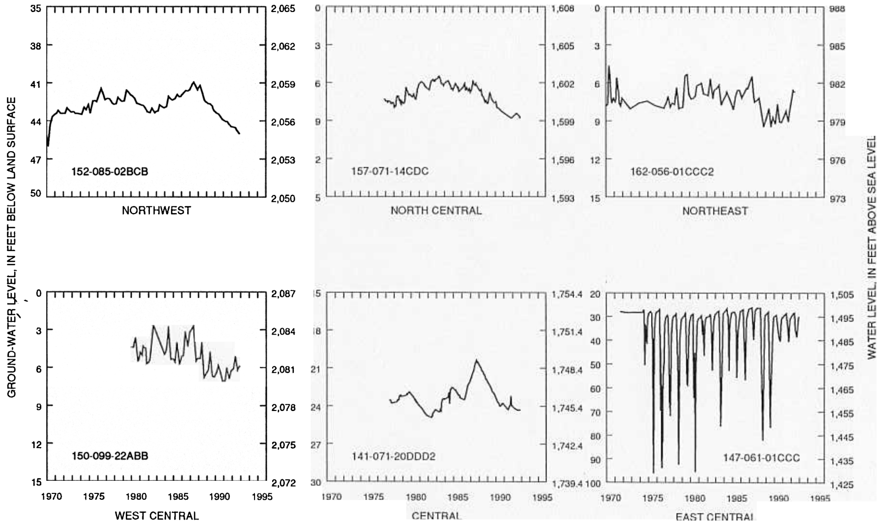
Figure 9. Ground-water levels in selected wells during 1970-92 for northwest, north-central, northeast, west-central, central, and east-central climatic divisions in North Dakota.
