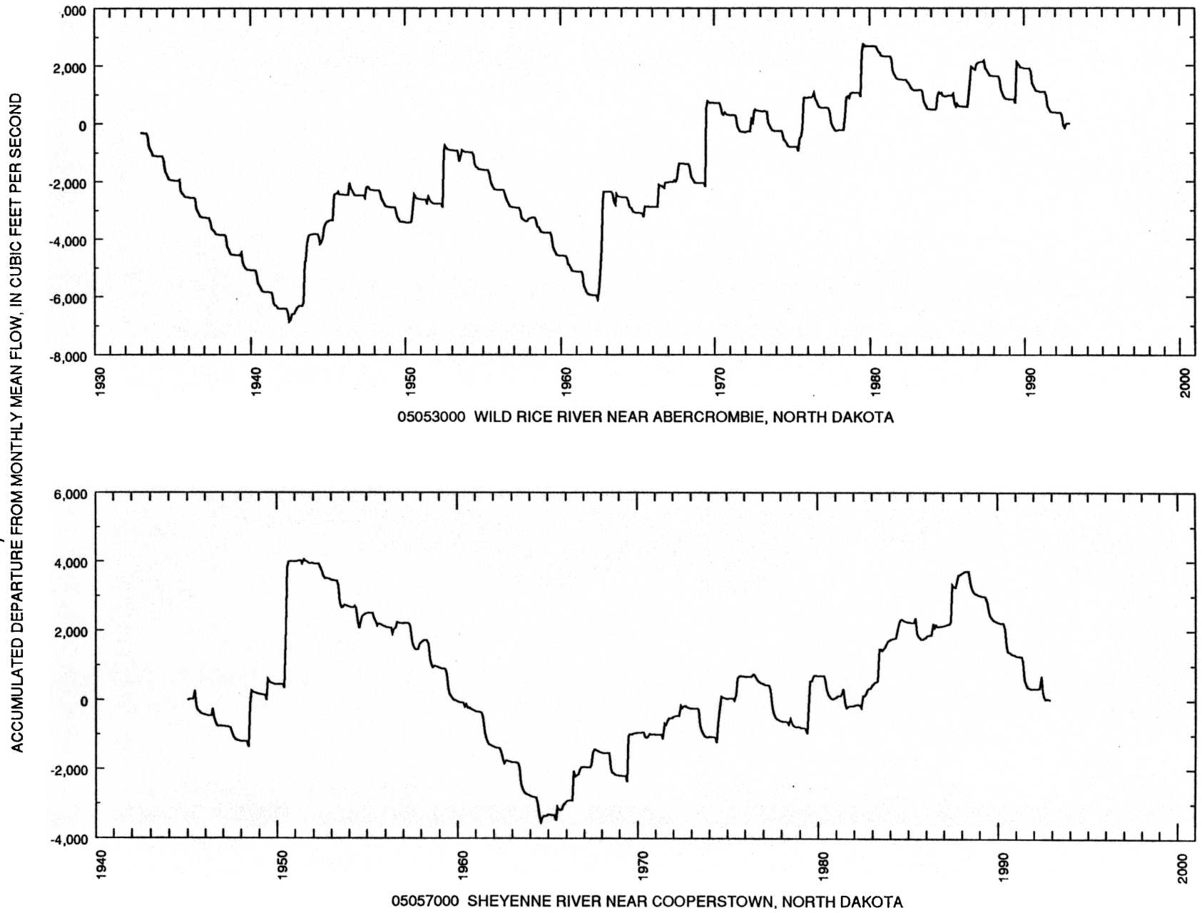
Figure 16. Accumulated departure from mean monthly flow for six representative streamflow-gaging stations in North Dakota
