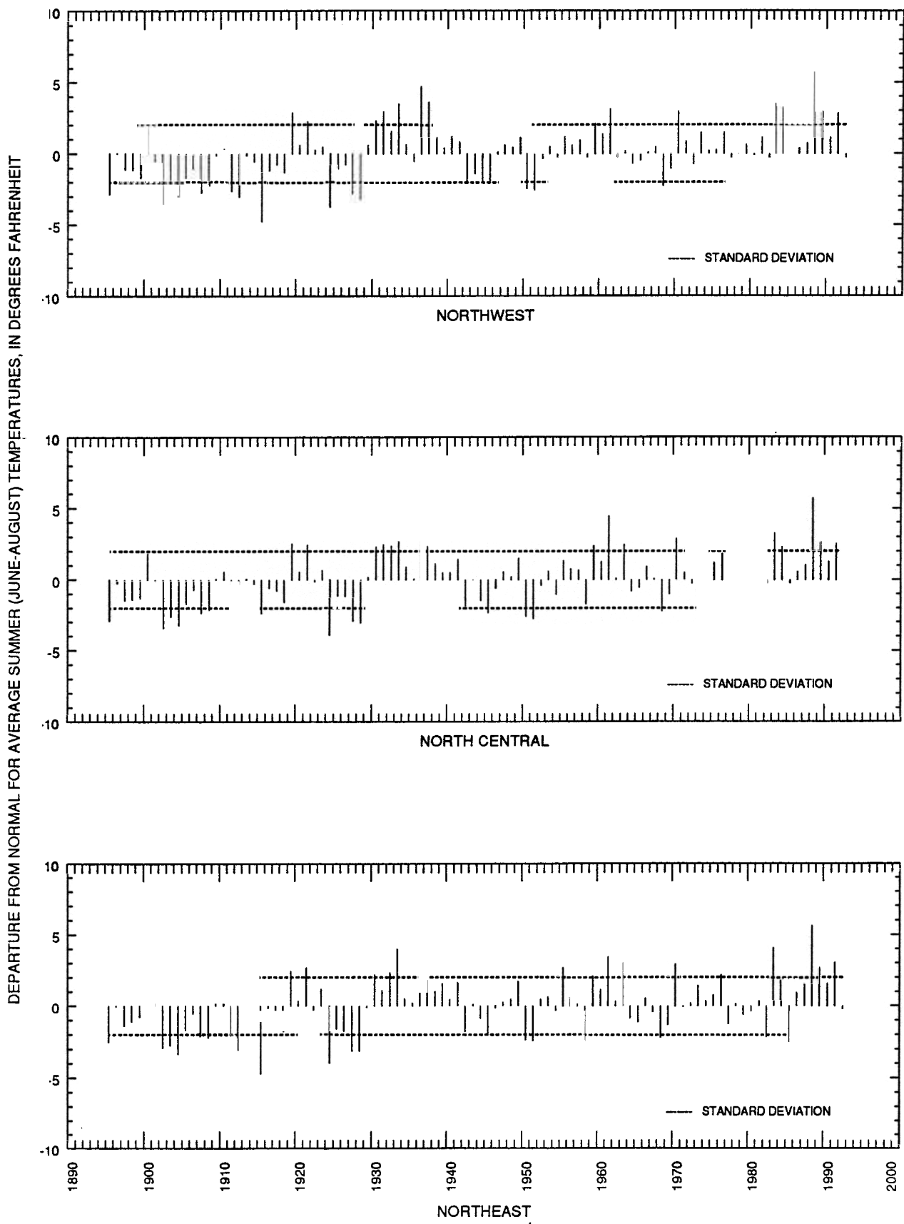
Figure 5. Departure from normal for average summer (June-August) temperatures from 1895 through 1992 for each climatic division in North Dakota.
