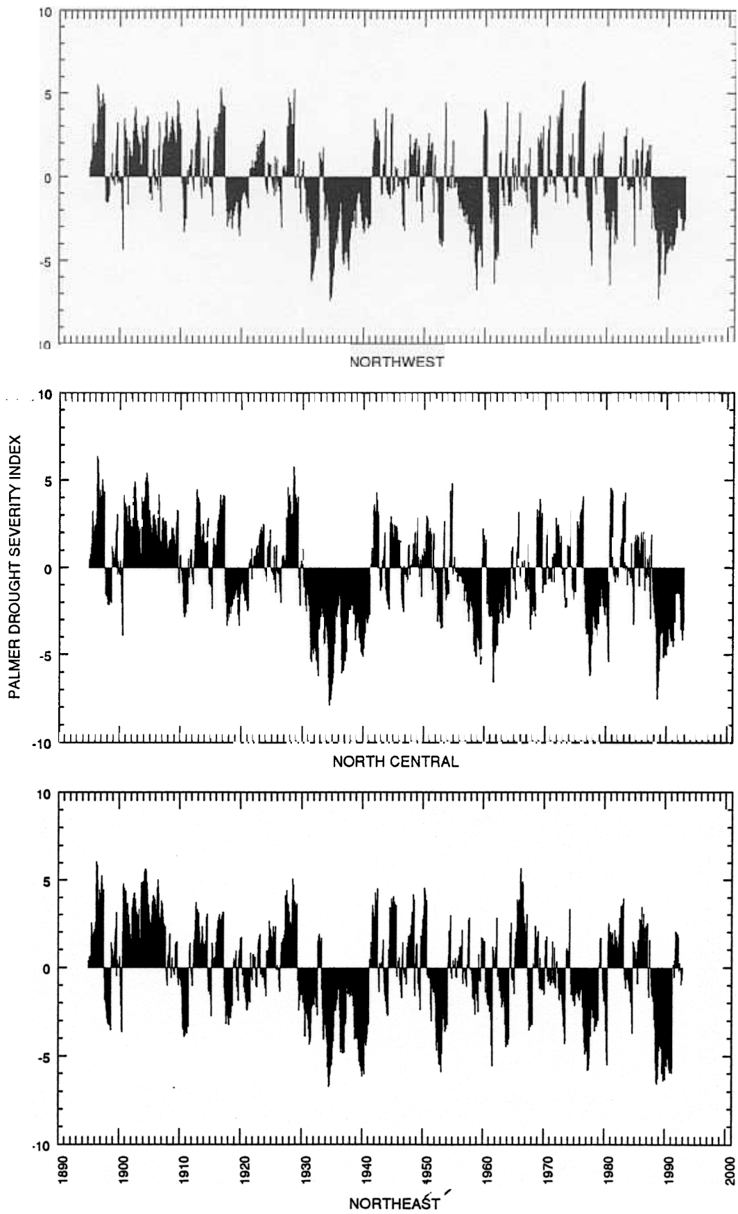
Figure 15. Palmer Drought Severity Index for each climatic division in North Dakota
