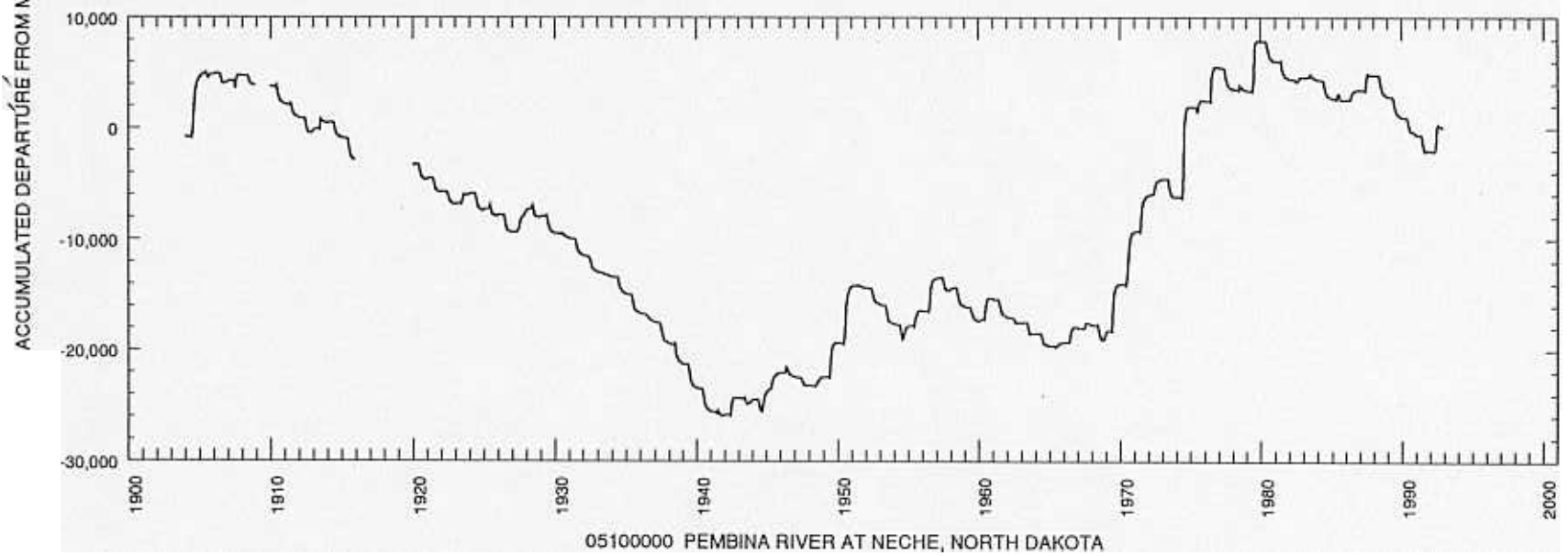
Figure 16. Accumulated departure from mean monthly flow for six representative streamflow-gaging stations in North Dakota--Continued.
