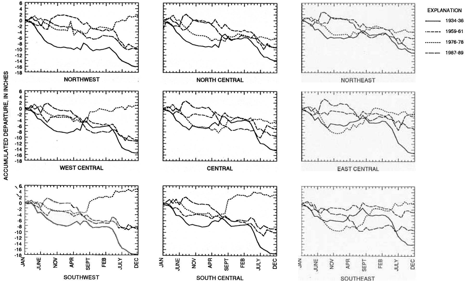
Figure 14. Accumulated departure from mean monthly precipitation for a 3-year period for each climatic division in North Dakota.
