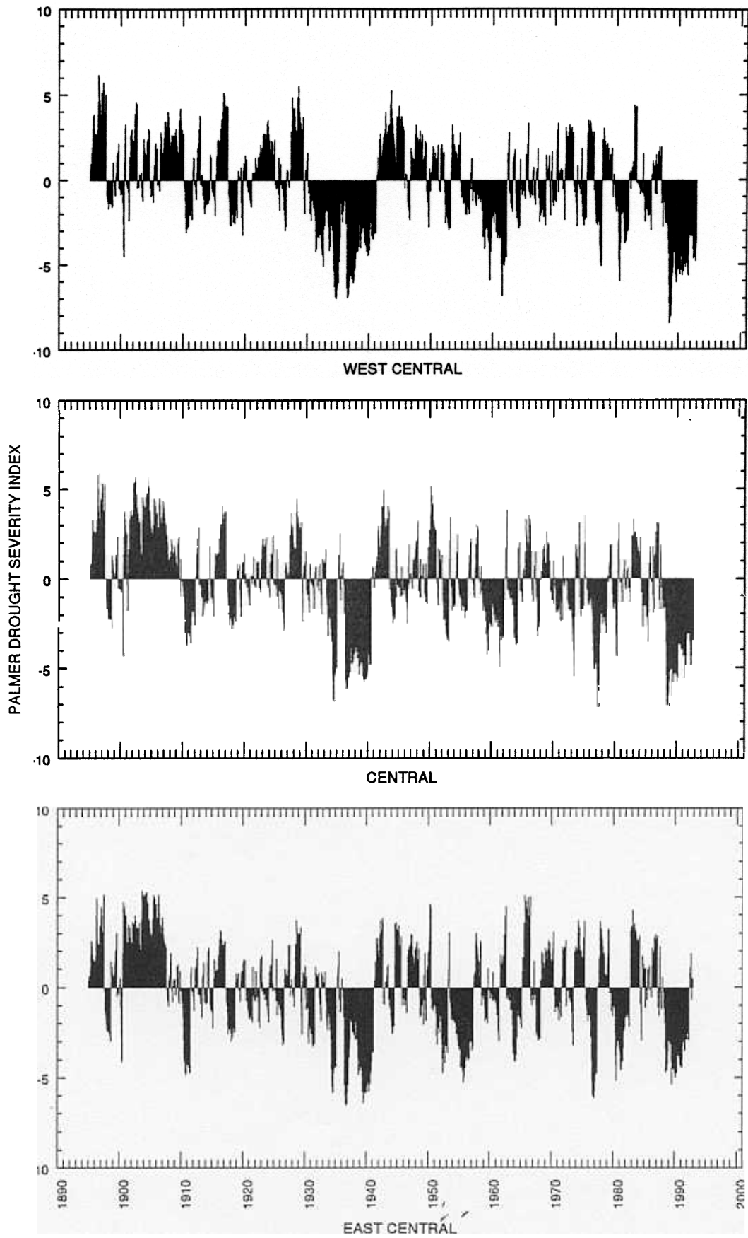
Figure 15. Palmer Drought Severity Index for each climatic division in North Dakota--Continued
