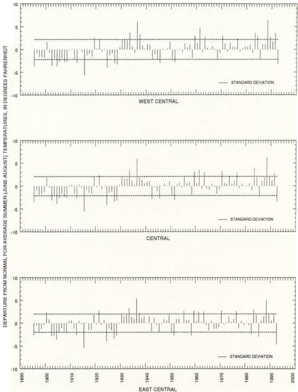
Figure 5. Departure from normal for average summer (June-August) temperatures from 1895 through 1992 for each climatic division in North Dakota--Continued.
