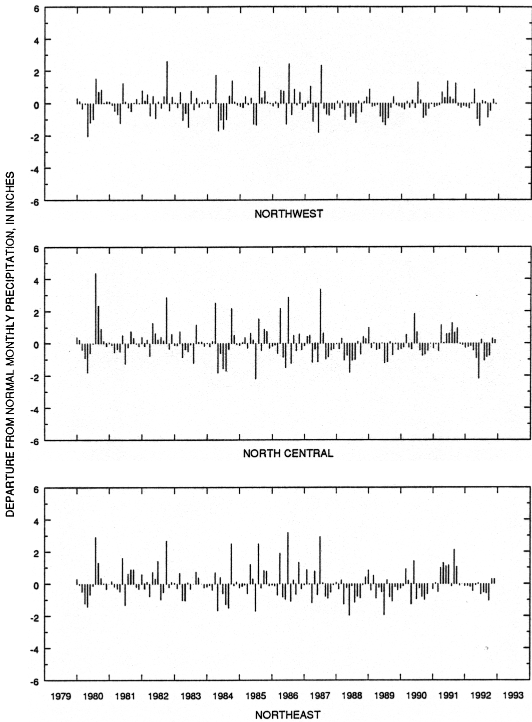
Figure 2. Departure from normal monthly precipitation during 1980-92 for each climatic division in North Dakota.
