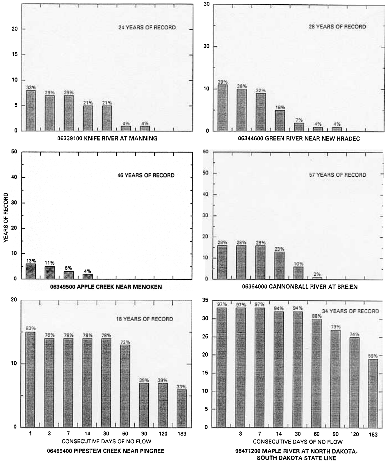
Figure 8. Percentage of years in period of record in which consecutive days of no flow occurred at selected streamflow-gaging stations in North Dakota--Continued.
