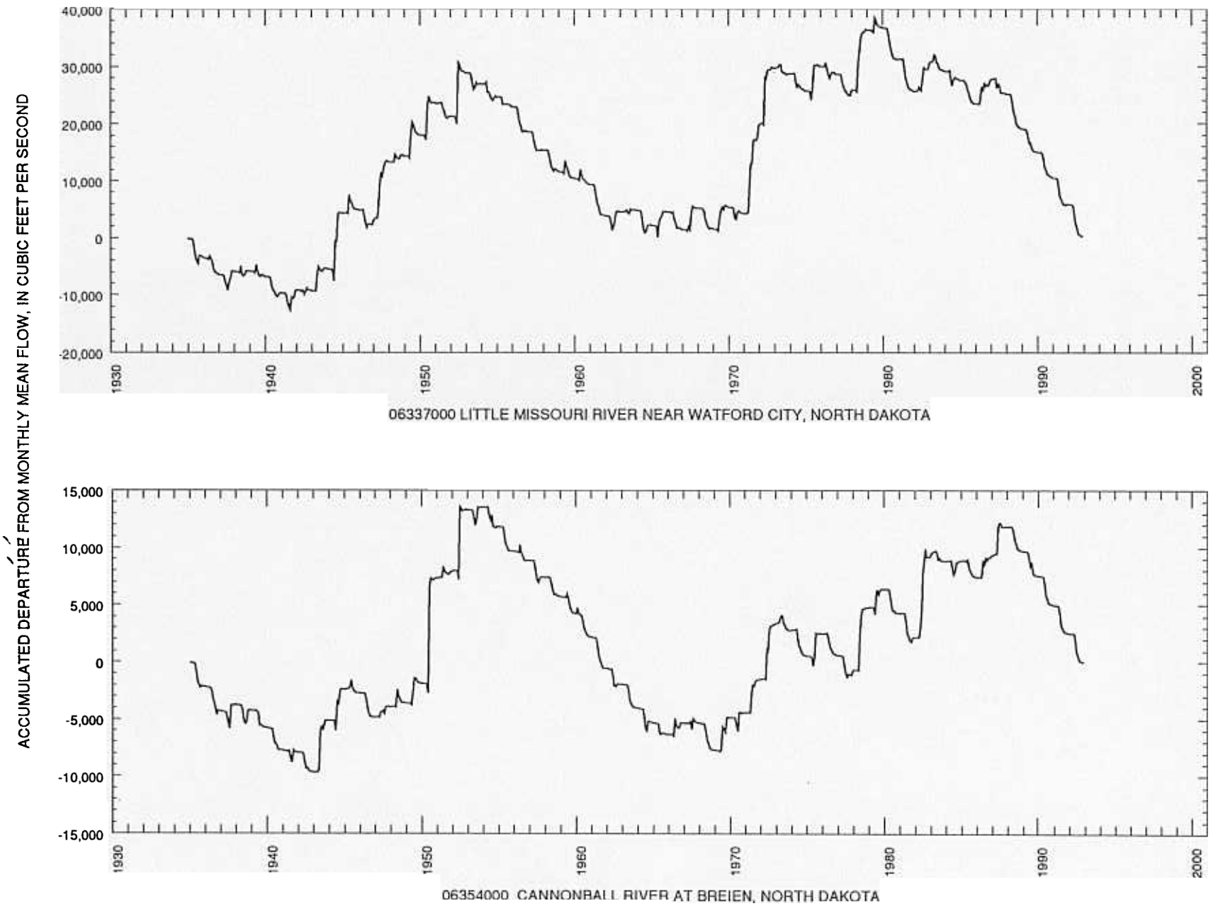
Figure 16. Accumulated departure from mean monthly flow for six representative streamflow-gaging stations in North Dakota--Continued.
