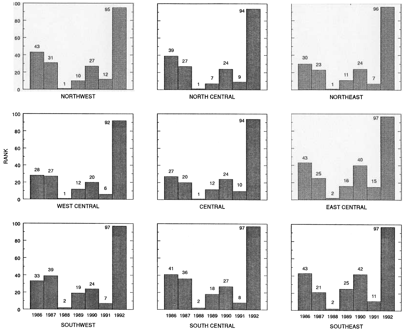
Figure 6. Rank of 1986-92 average summer (June-August) temperatures from 1895 through 1992 for each climatic division in North Dakota (1 indicates warmest summer, 98 indicates coolest summer).
