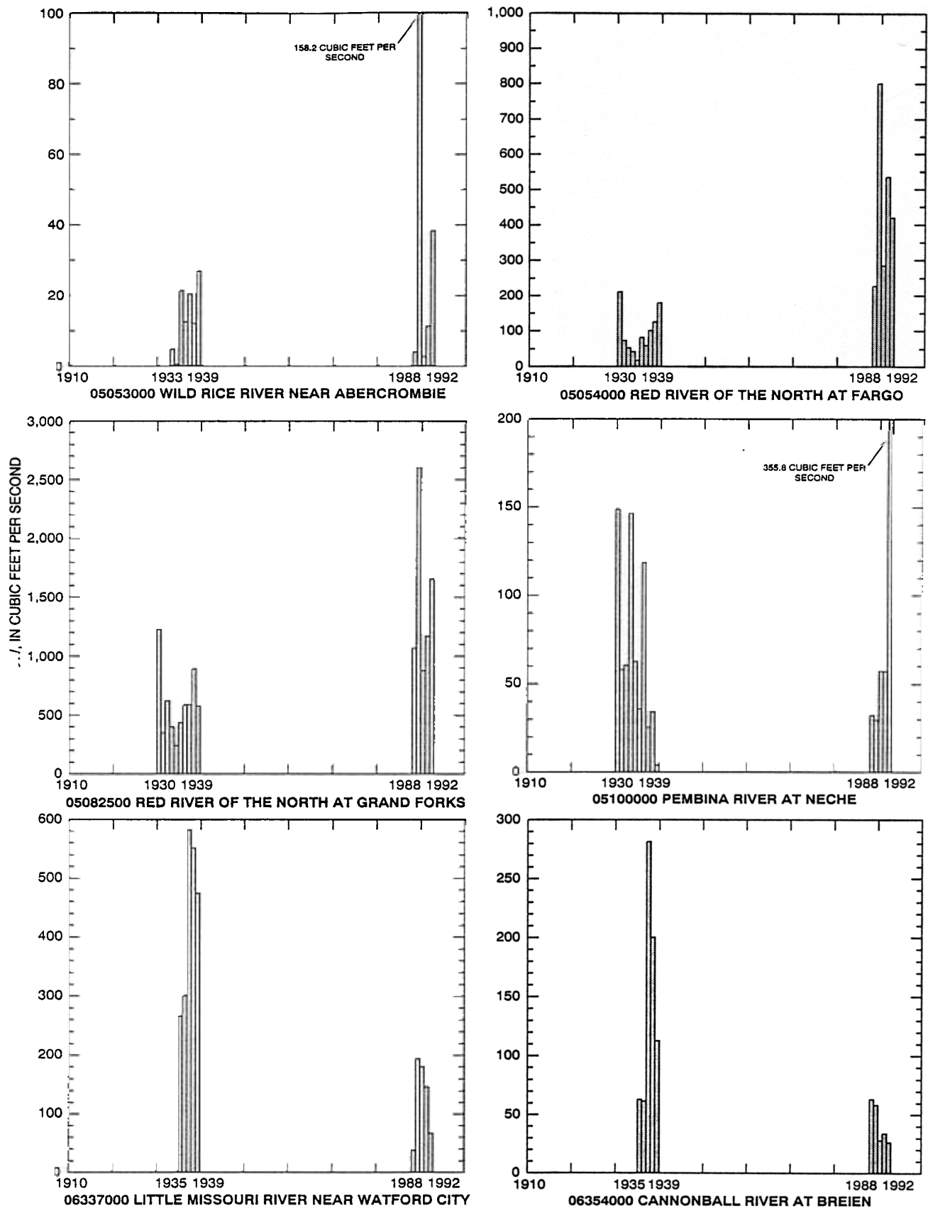
Figure 17. Average annual streamflows for selected gaging stations in North Dakota during water years of the 1930's and water years from 1988 through 1992.
