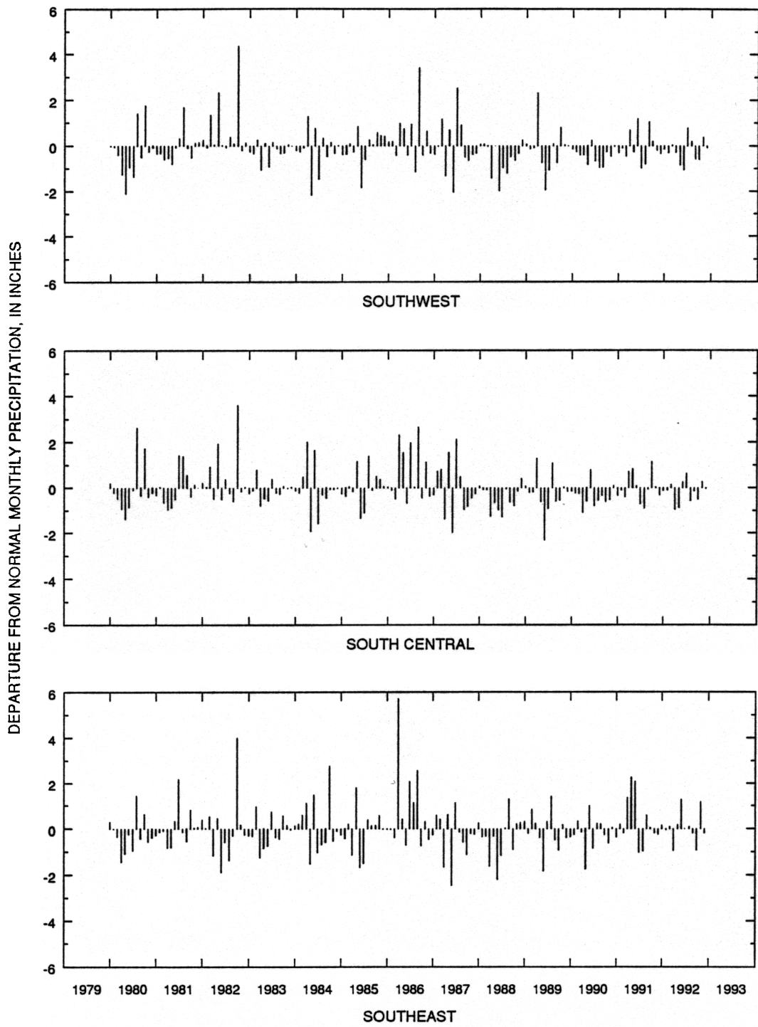
Figure 2. Departure from normal monthly precipitation during 1980-92 for each climatic division in North Dakota--Continued.
