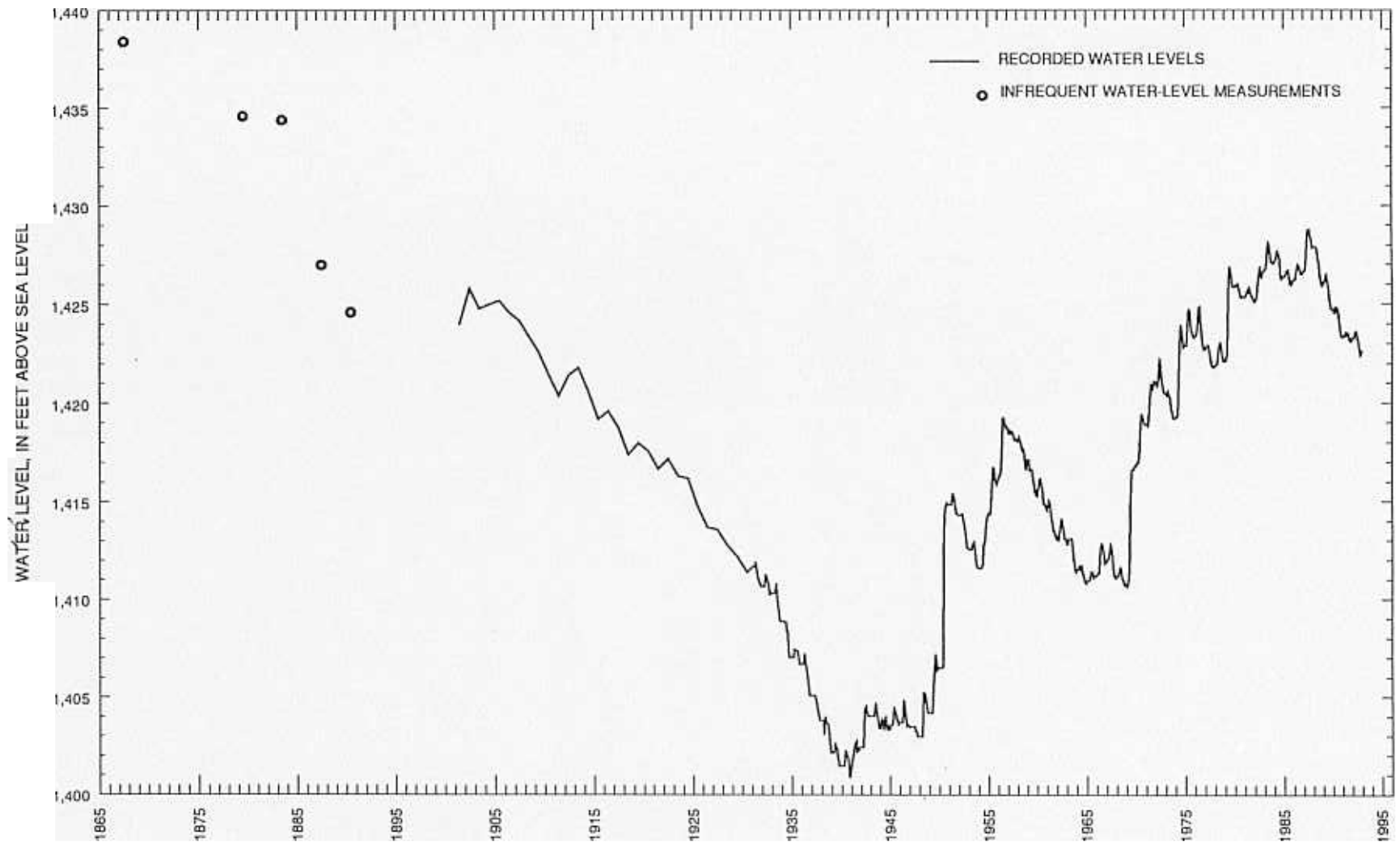
Figure 18. Water levels of Devils Lake, North Dakota, 1867-1992.
