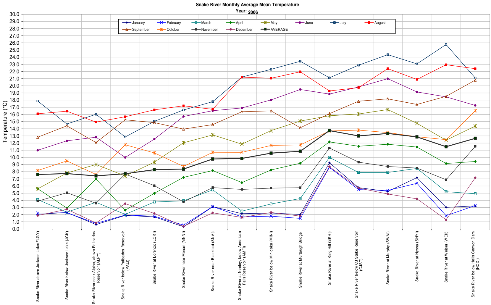
Figure 4-2. Average monthly water temperature at locations along the Snake River - 2006.
