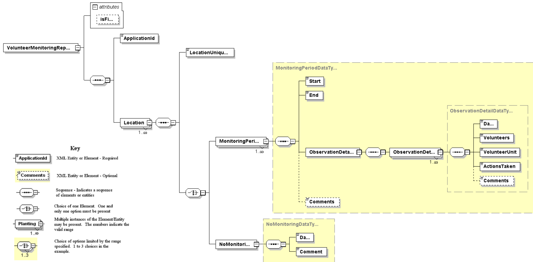
Figure 2 - XSD Diagram
