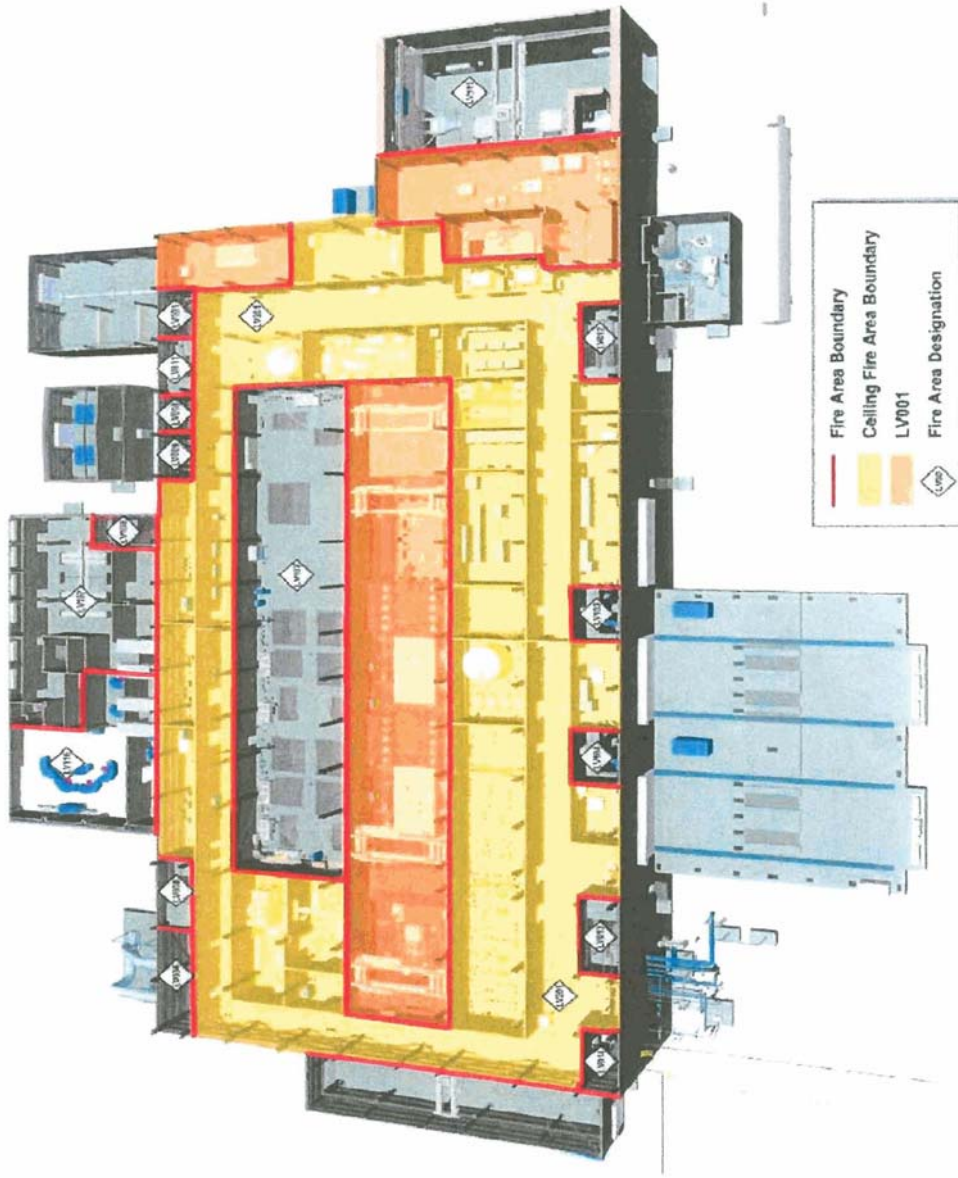
Figure 8 LAW Building Fire Boundaries at Elevation 28 Ft
