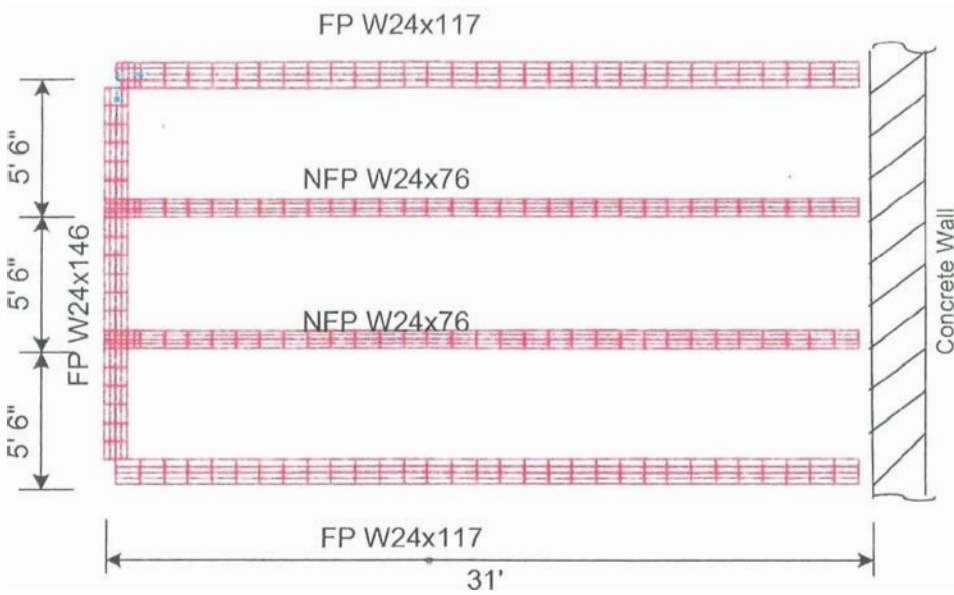
Figure 18 Plan View of Case 1c (One NFP W24x76 heated)
