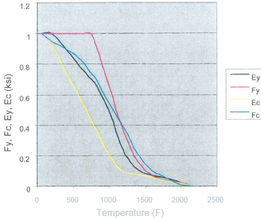
Figure 16 Rate of Decline of F_y , F_c , E_y , E_c v. Temperature
