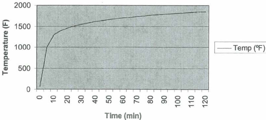
Figure 14 Time-Temperature Curve
