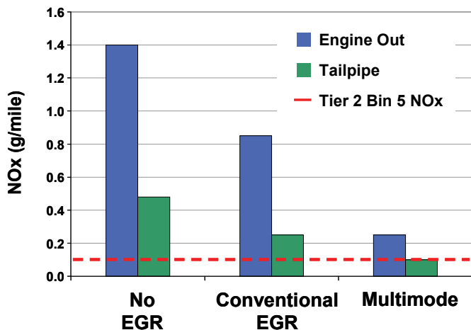
Figure 2: NO x emissions for conventional vs multimode operation with a DPF-LNT emission control system.
