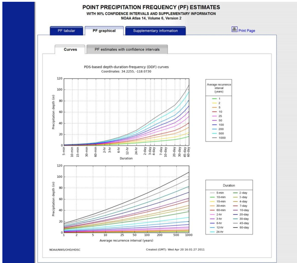
Figure 13. New format – precipitation frequency estimates displayed in graphic form for the same location used in Figure 12. This is displayed by clicking on the “PF graphical” tab.
