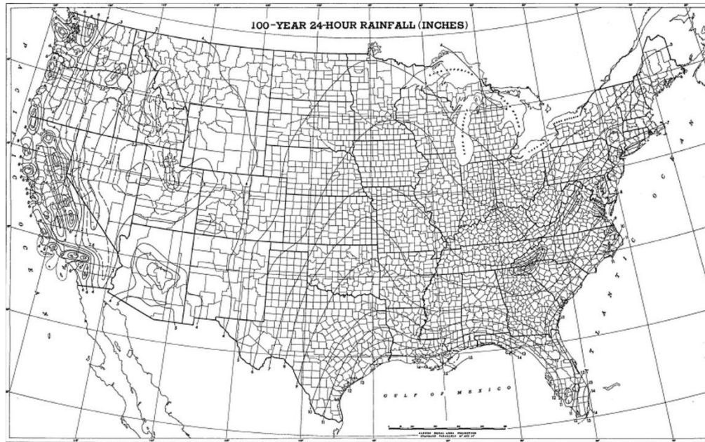
Figure 14. Old format – national map with lines of constant depth for 100-year, 24 hour precipitation, scanned from Technical Paper No. 40 and provided via the Precipitation Frequency Data Server.
