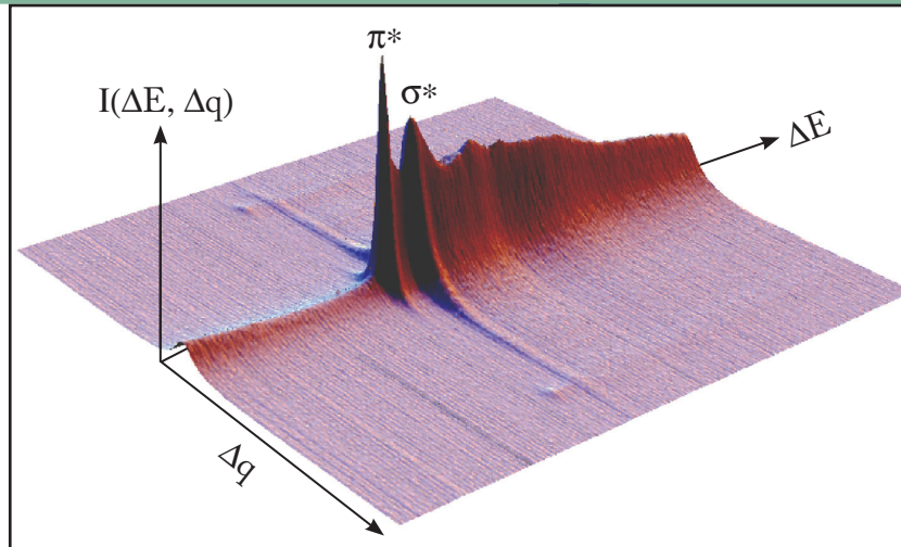
High-resolution momentum resolved spectroscopy developed within the EMC allows researchers to investigate the orientation dependence of the electronic properties of materials.
