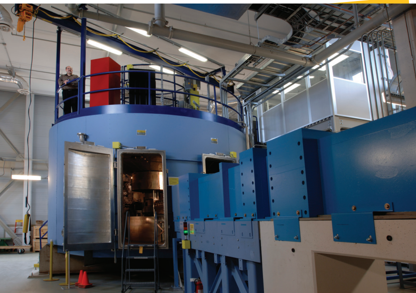
Outside view of the backscattering reflectometer. For a sense of the size and scale of neutron scattering instrumentation, note the man standing on the top platform.
