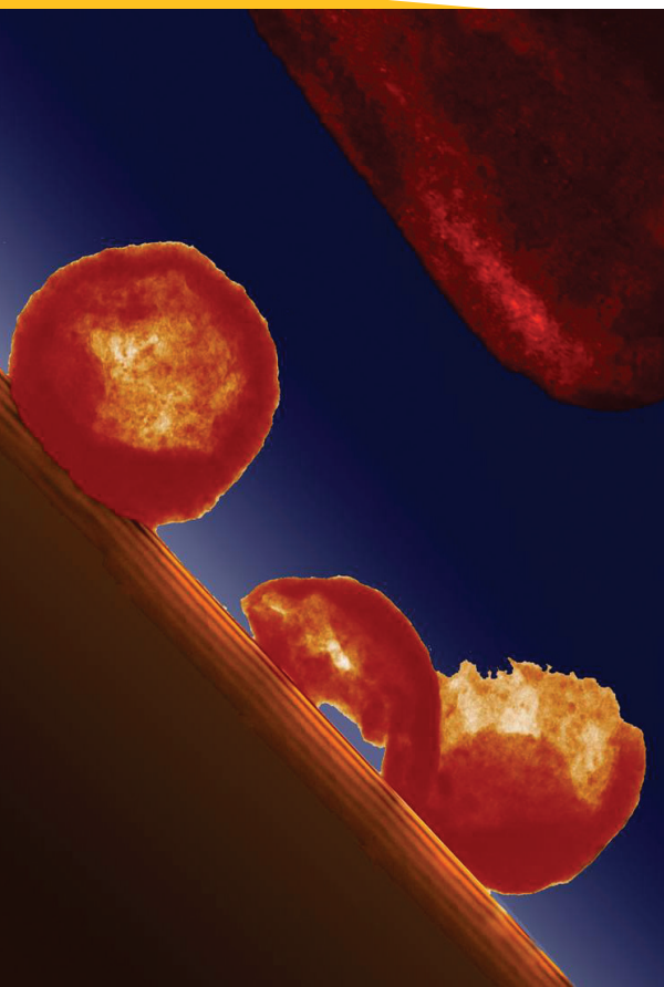
Before and after in-situ deformation experiment of 200-nm-diameter hollow nanospheres of cadmium sulfide.
