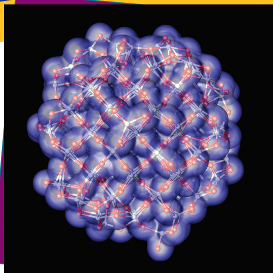
Structure and charge density of a 2-nm titanium dioxide nanoparticle from ab initio calculations. (Courtesy of Paul Kent, Oak Ridge National Laboratory, and James Kubicki, Penn State University.)
