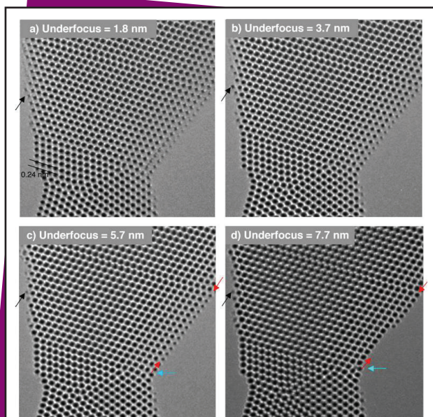
Series of atomic resolution images recorded on TEAM 0.5, showing a nanobridge connecting two gold crystals. Arrows highlight atomic rearrangements.
