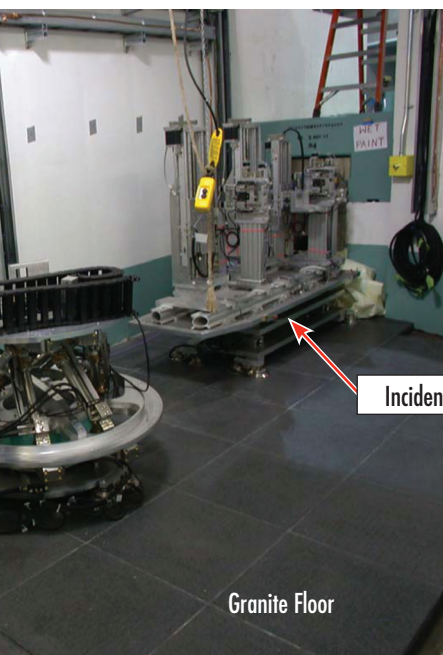
Magnetism Reflectometer. Hardware items depicted here, from right to left, are the incident optics, hexapod sample support, and detector tables.
