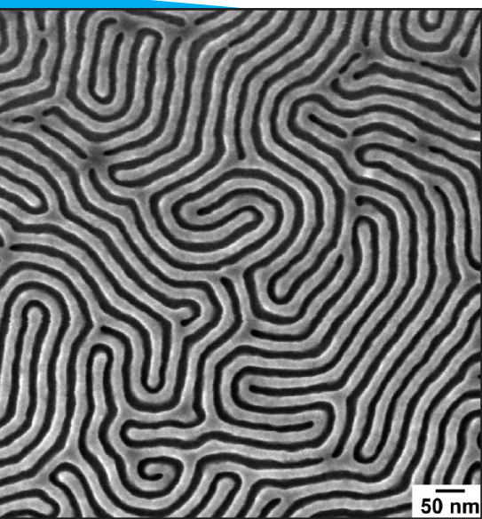
Scanning electron microscope image of a lamellar-phase block copolymer thin film. This self-assembled striped pattern has feature sizes of 18 nanometers with 36 nanometer period spacing.
