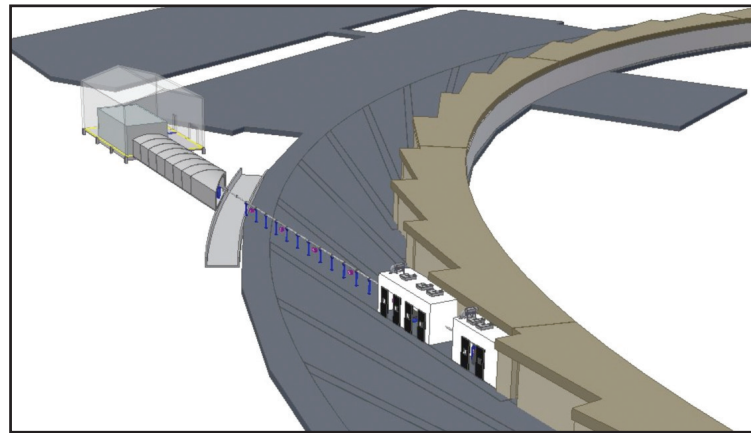
Schematic view of the hard x-ray nanoprobe beamline, with a remote satellite building at \sim 100 m from the source.
