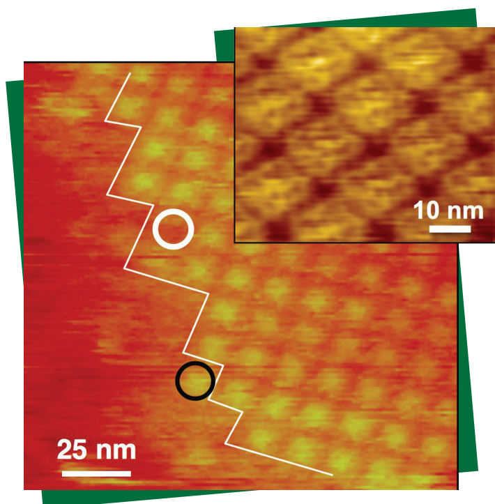
In situ AFM image of S-layer proteins during self-assembly in fluid. Black (white) circles indicate newly attached (detached) proteins. Inset shows high-resolution image revealing tetrameric substructure of growth units.
