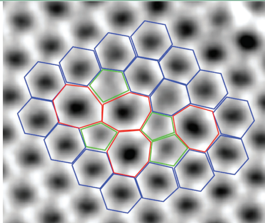
Using a monochromated beam at 80kV, TEAM 0.5 is able to resolve atomic defects such as this arrangement of 5- and 7-fold rings in graphene sheets only one atom thick. (after Meyer et al. NanoLetters 2008)
