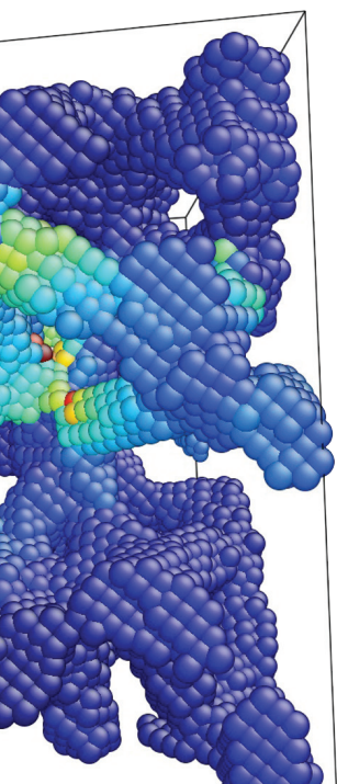
Computer generated model of a copper nanofoam deformed under volume conserving planar strain.
