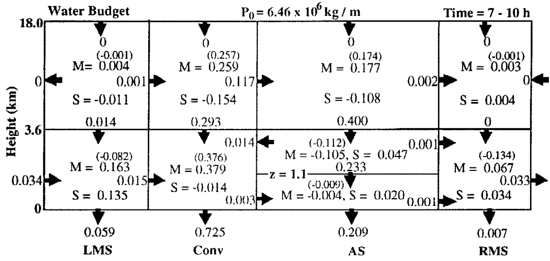
Figure 3. The water budget of the control run over the whole domain at the mature stage. All quantities are normalized by the total surface precipitation ( P_0 ). M represents the net microphysical production; S, the storage term; arrows, the horizontal and vertical transport; LMS and RMS, leading and rear marine stratus; Conv, convective; and AS, anvil stratus.
