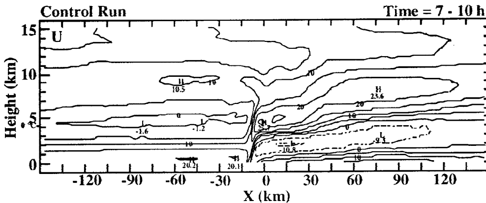
Figure 2. Model estimated (instantaneous) radar reflectivity (dBZ) plotted at 10-dBZ intervals. Shading represents the bright melting band.
