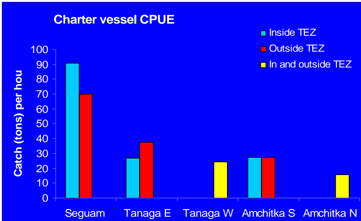
Figure 2, Average Charter Vessel CPUE (catch in tons per hour trawled) from 2002-2003 per study area.
