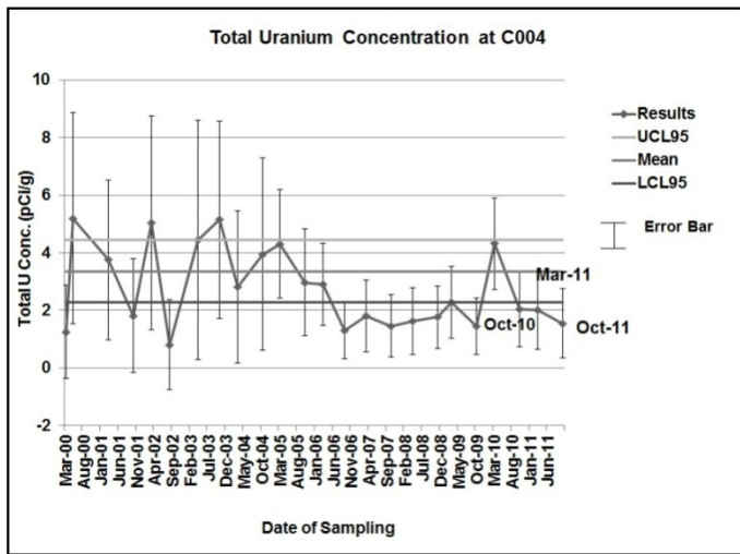
Figure 3-5. Total U Concentrations in Surface Water Versus Sampling Date
