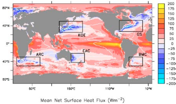
Figure 1. Climatological mean net surface heat flux into the ocean from the OAFLEX product [43]. White contours indicate mean dynamic sea level [53].
