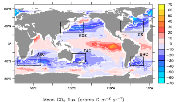
Figure 2. Climatological mean annual sea-air CO 2 flux (grams C m -2 yr -1 ) for the reference year 2000 (non-El Niño conditions). Adapted from [34]. White contours indicate mean dynamic sea level [53].
