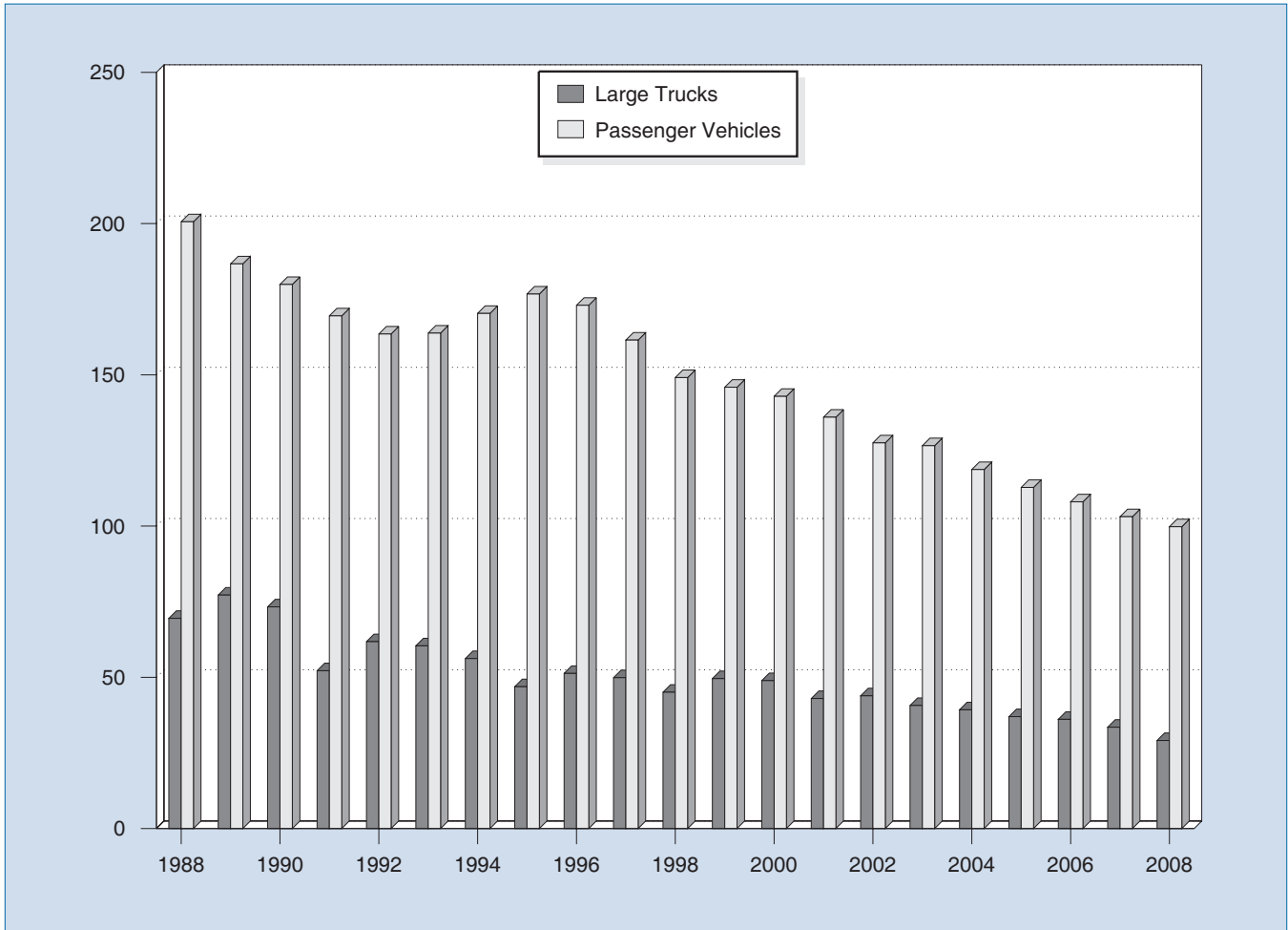
Figure 4. Large Trucks and Passenger Vehicles Involved in Injury Crashes per 100 Million Vehicle Miles Traveled, 1988-2008
