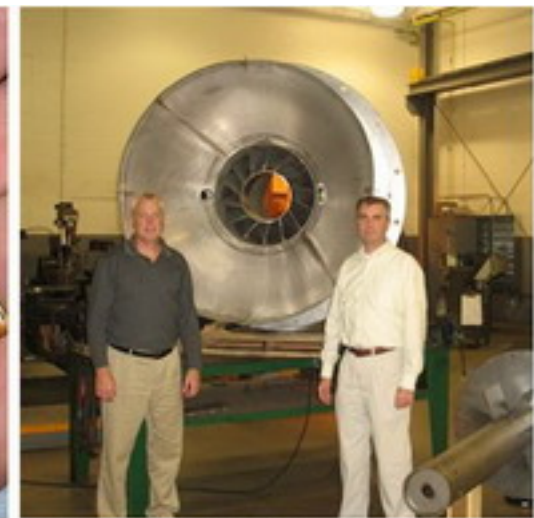
28" burner (44 MW, 150 MBtu/hr)
