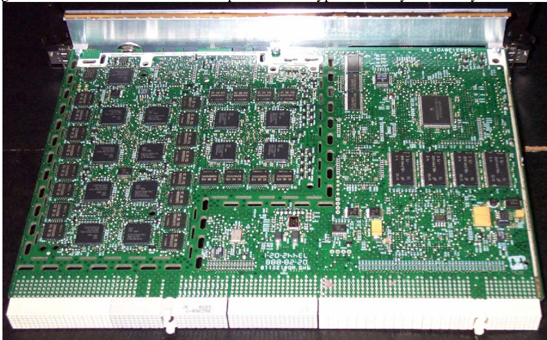
Figure 2: MGE SCCE back w/o tamper shield. Crypto boundary defined by dashed 'line'.
