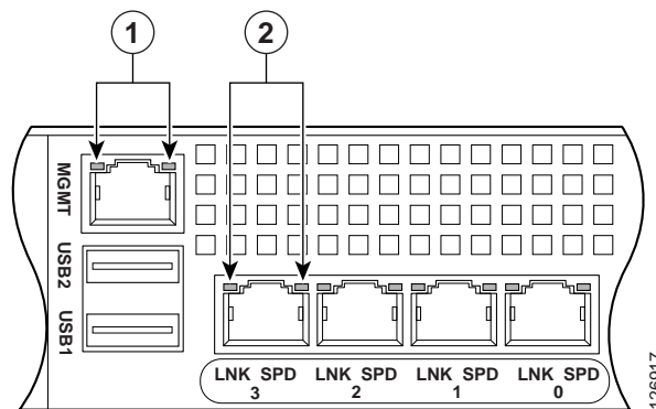
Figure 3 ASA 5500 Adaptive Security Appliance Rear Panel Link and Speed Indicator LEDs
