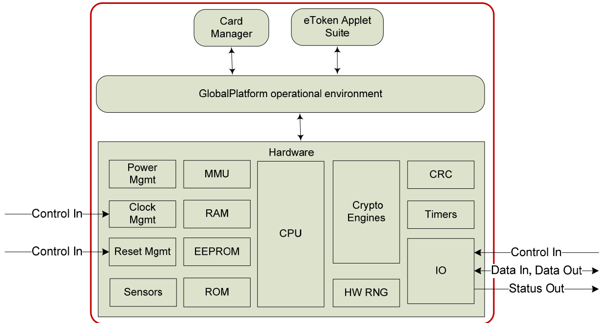
Figure 4 - Module Block Diagram
