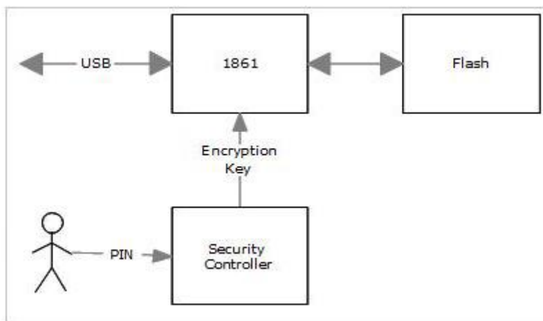
Figure 2 - Main component architecture of Aegis Secure Key
