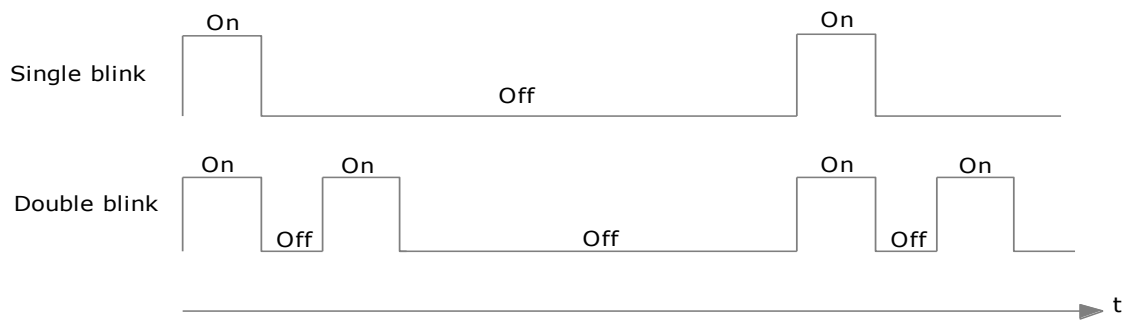
Figure 3 - Blinking patterns for user and crypto-officer
