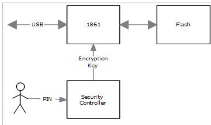
Figure 2 - Main component architecture of datashur
