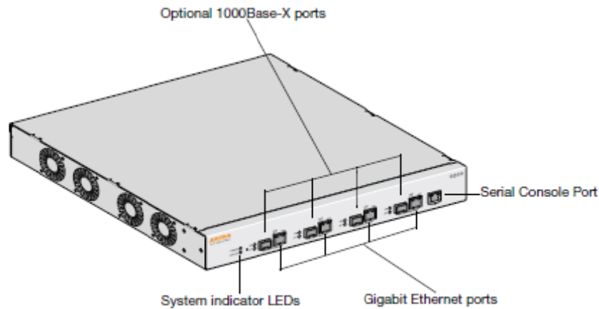
Figure 2 The Aruba 3000-series Controller Chassis
