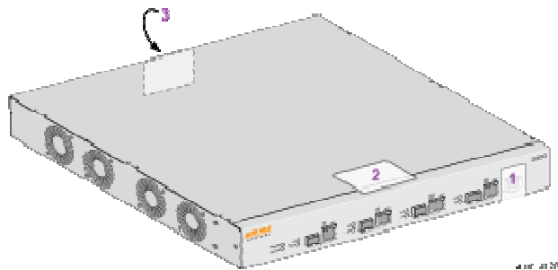
Figure 5 Required TELs for the Aruba 3000-series Controller
