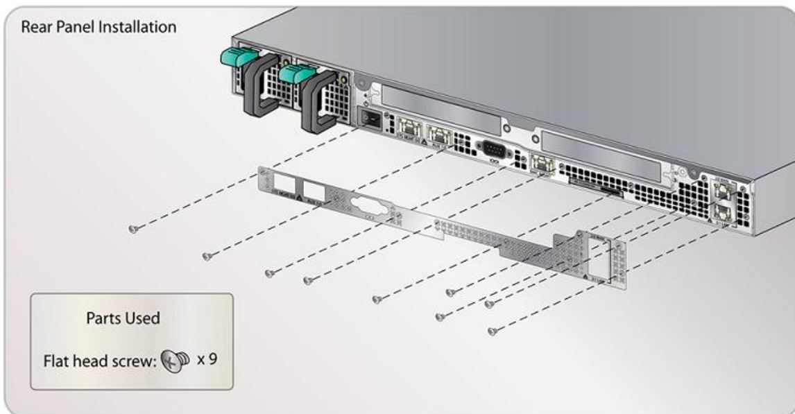
Figure 6 Rear Security Panel Installation
