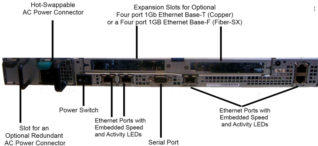
Figure 3 Connection Ports at the Rear of the ProxySG 900-10, 20, 30, 45, 55
