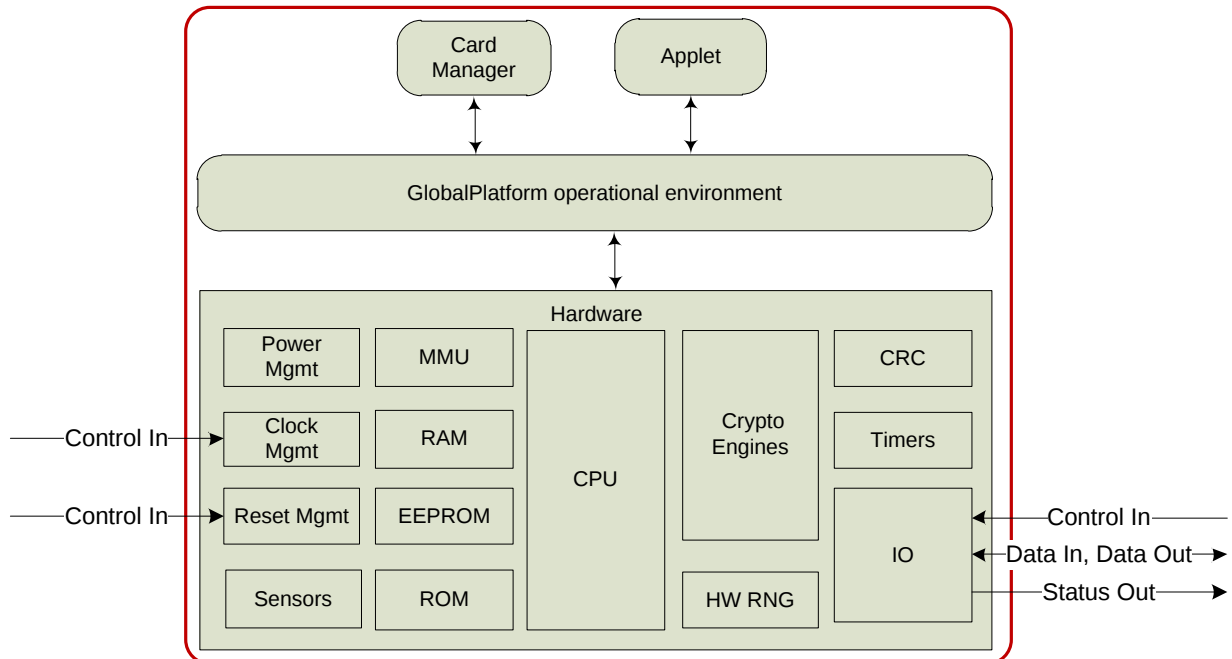
Figure 3 - Module Block Diagram
