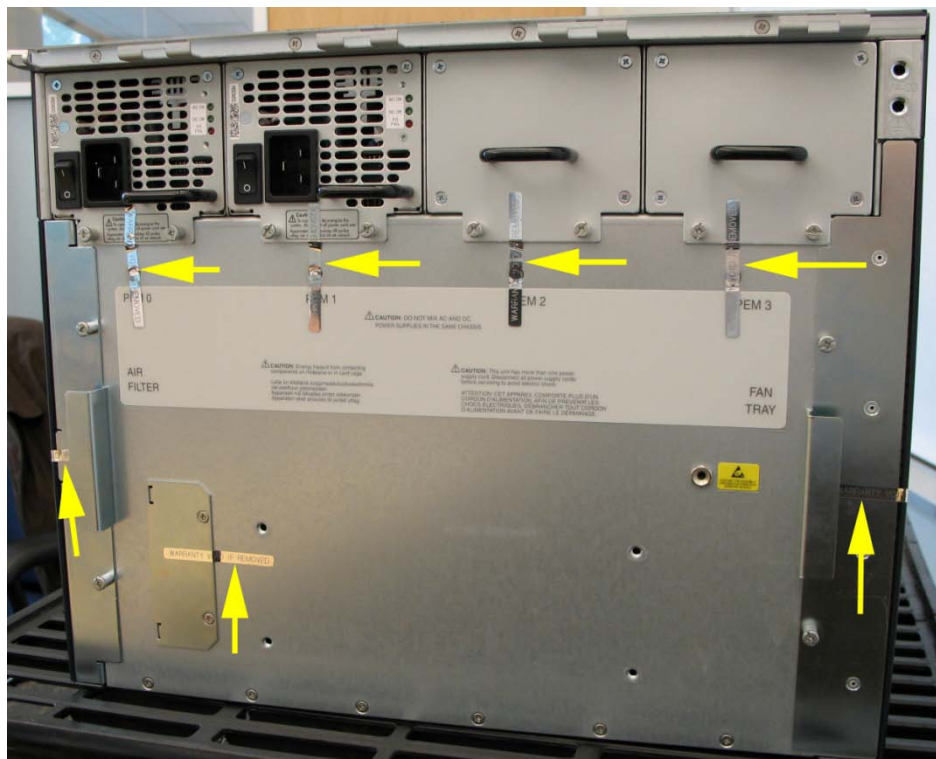
Figure 3. SRX5600 Tamper Evident Seal Location (Rear)
