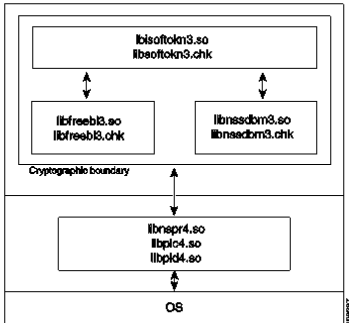
Figure 2 NSS PKCS #11 Interface
