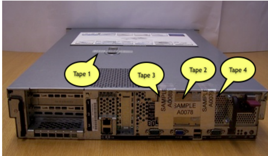
Illustration 5: tamper-evident security tape covering lock and cover latch, power supply bay and power supply
