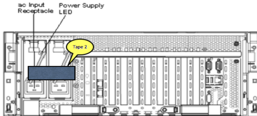
Illustration 11: tamper-evident tape covering dual rx360 power supplies and attaching to main casing
