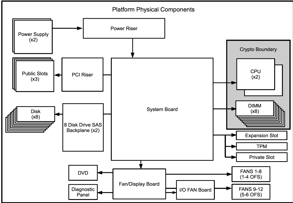
Illustration 6: Block Diagram of platform Physical Components indicating Crypto Boundary
