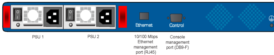
Figure 4-2 1600X435 Rear
