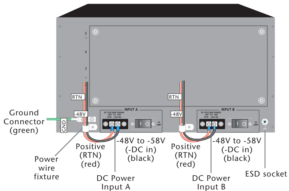
Figure 4: FortiGate-5050 Rear Panel
