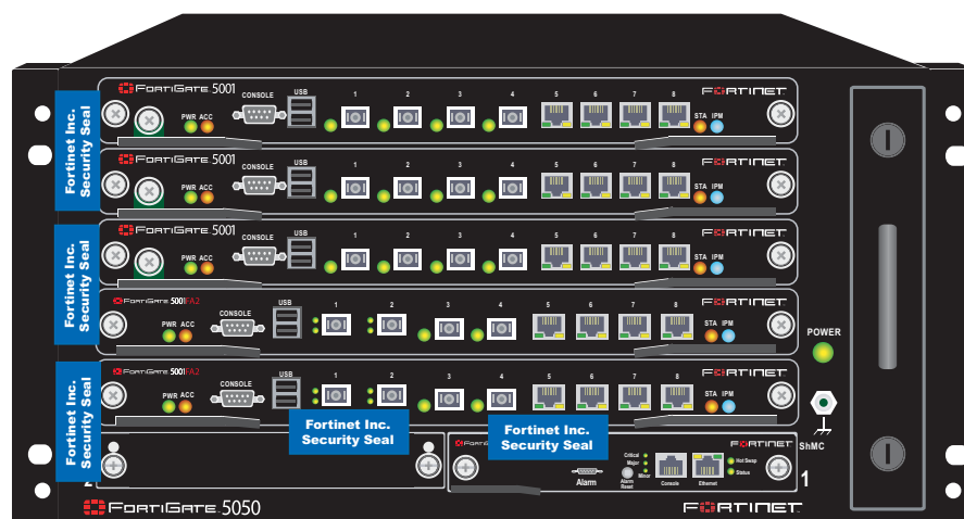
Figure 8: FortiGate-5050 front panel tamper seal placement
