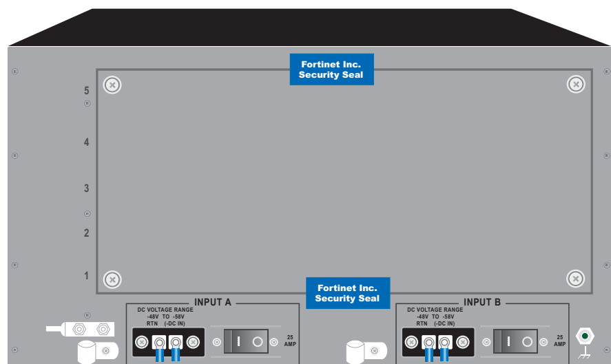
Figure 9: FortiGate-5050 rear panel tamper seal placement
