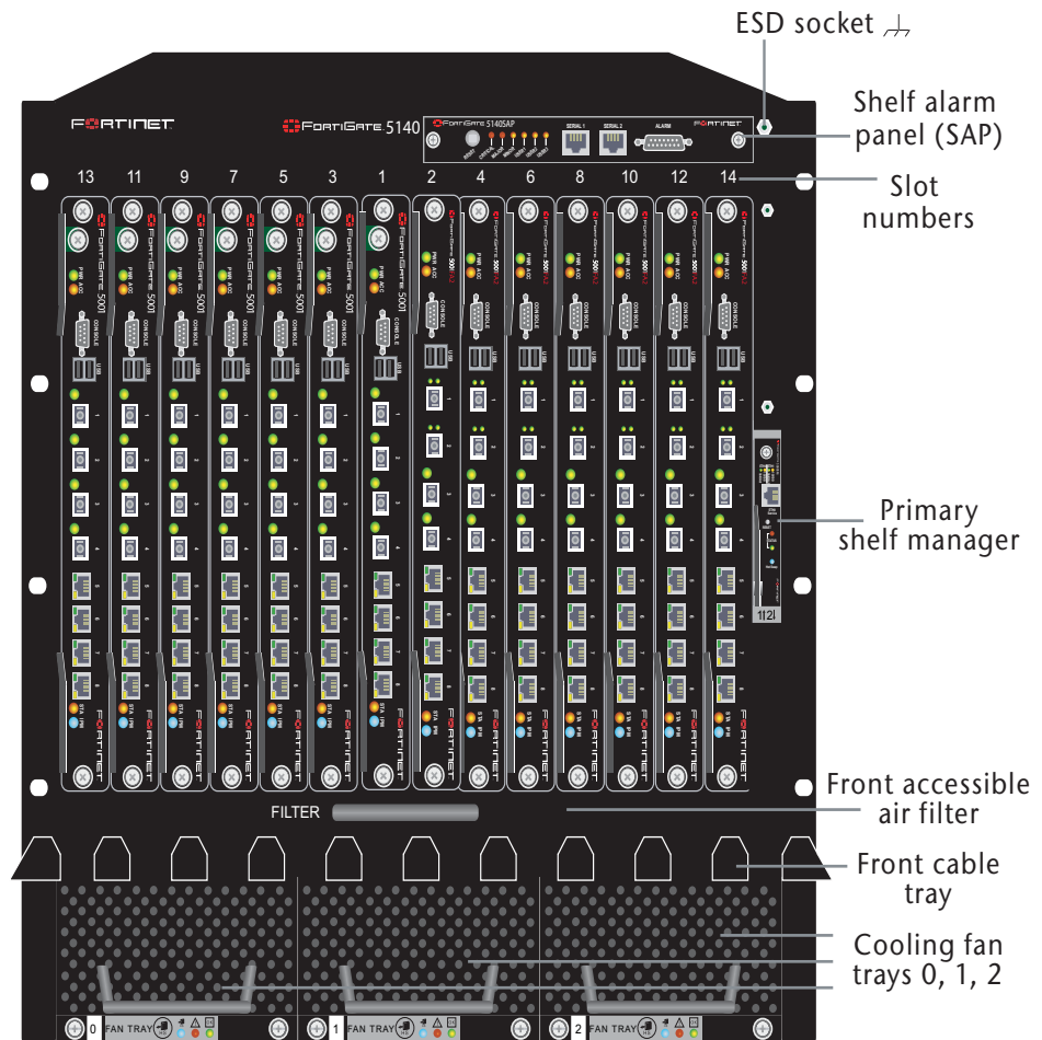
Figure 5: FortiGate-5140 Front Panel
