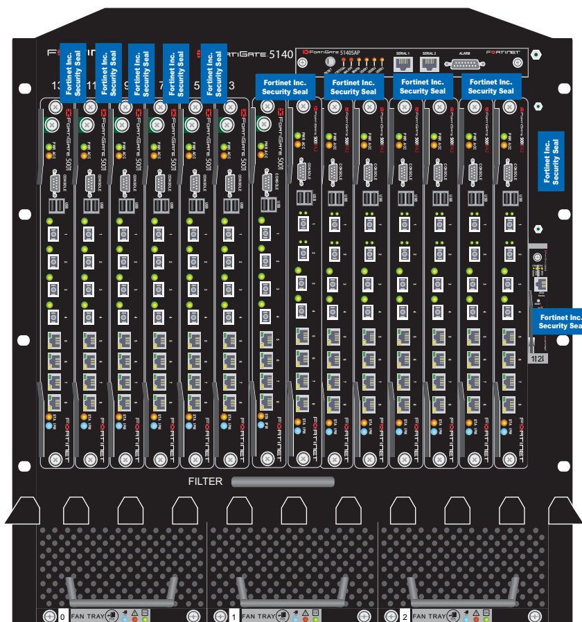
Figure 11: FortiGate-5140 front panel tamper seal placement
