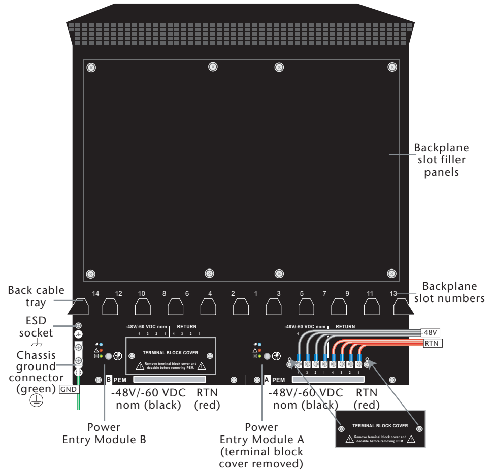
Figure 6: FortiGate-5140 Rear Panel
