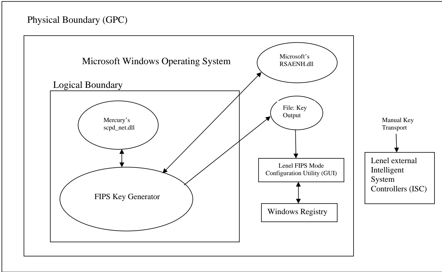
Figure 2 – Diagram of the FIPS Key Generator Module
