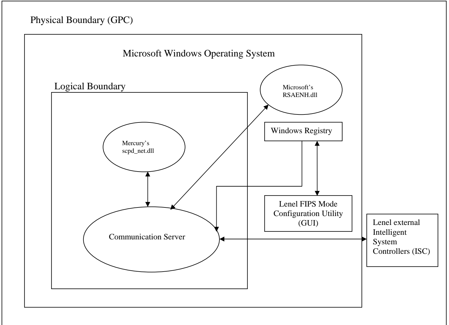
Figure 1 – Diagram of the Communication Server Module
