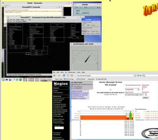
FIG. 2: This figure gives an idea about LivEPICS GUI
