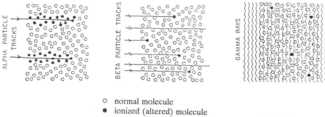
Figure G. Ionizing potentials for alpha, beta, and gamma radiation.
