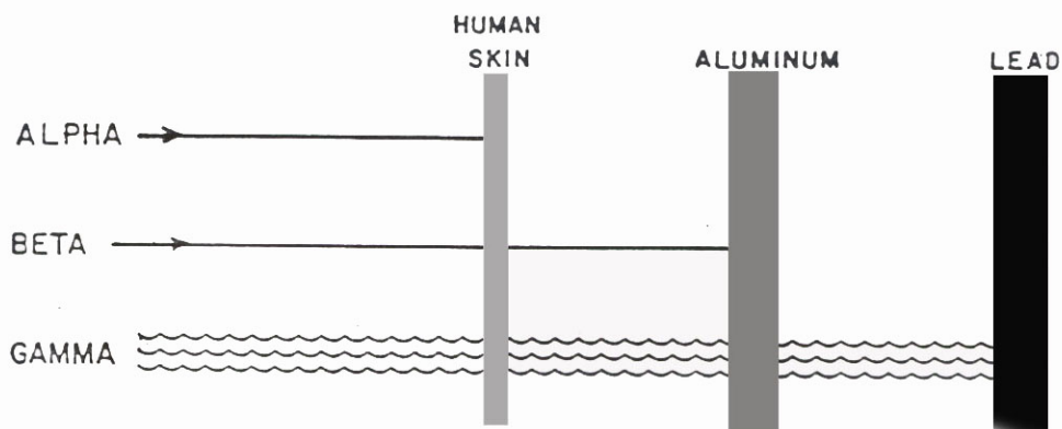
Figure F. Penetrating powers of alpha, beta, and gamma radiation.
