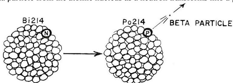
Figure D. Beta decay of Bismuth-214 to Polonium-214 (orbiting electrons not shown).
