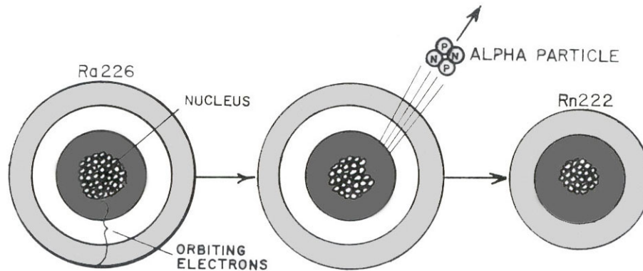
Figure 4. Conceptual Illustration - Alpha decay of Radium-226 to Radon-222
