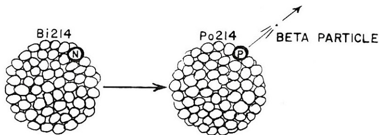
Figure 5. Conceptual Illustration - Beta decay of Bismuth-214 nucleus to Polonium-214 nucleus
