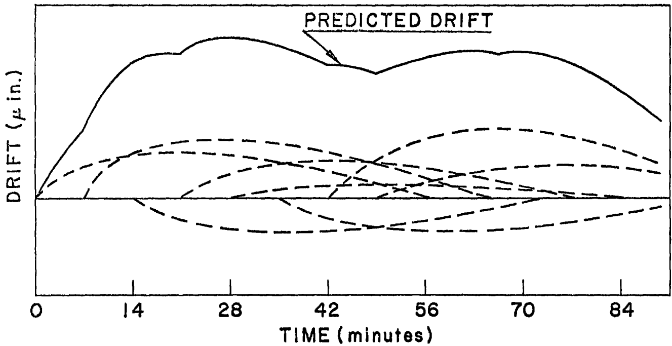
Fig. C-2. Graphical addition of drift components.
