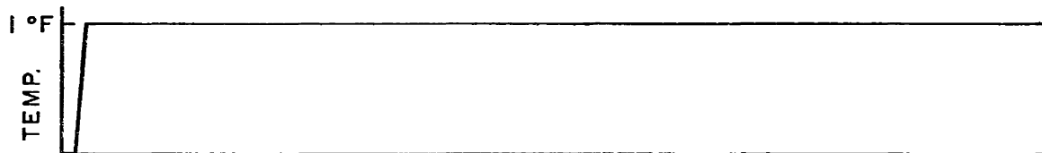
Fig. 7. Step input response on 15-inch Sheffield rotary contour gage No. 2.
