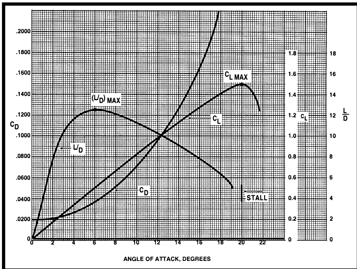
FIGURE 19.—Angle-of-Attack Chart.
