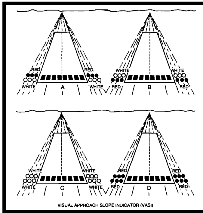
FIGURE 65.—VASI Illustrations.
