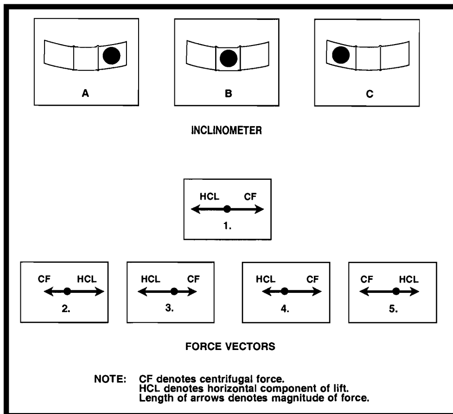
FIGURE 22.—Force Vectors.
