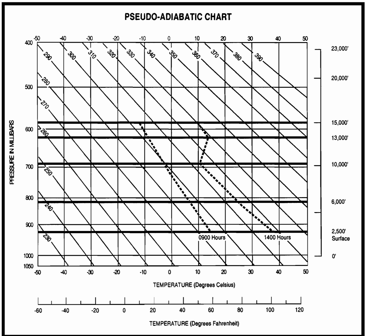
FIGURE 2.—Pseudo-Adiabatic Chart.
