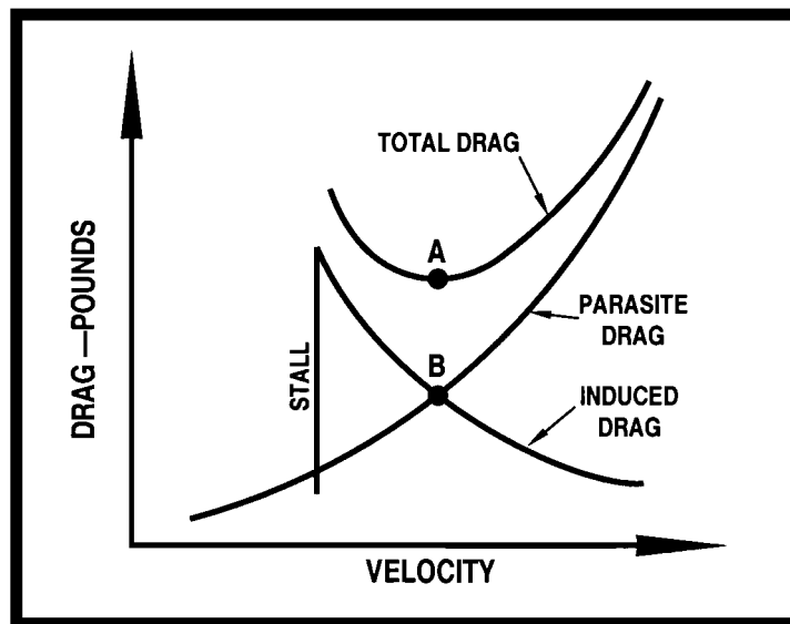
FIGURE 20.—Drag Chart.
