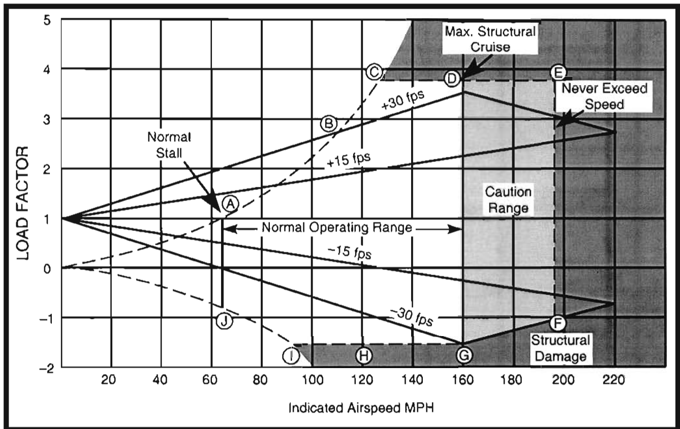
FIGURE 68.—Velocity vs. G-Loads.
