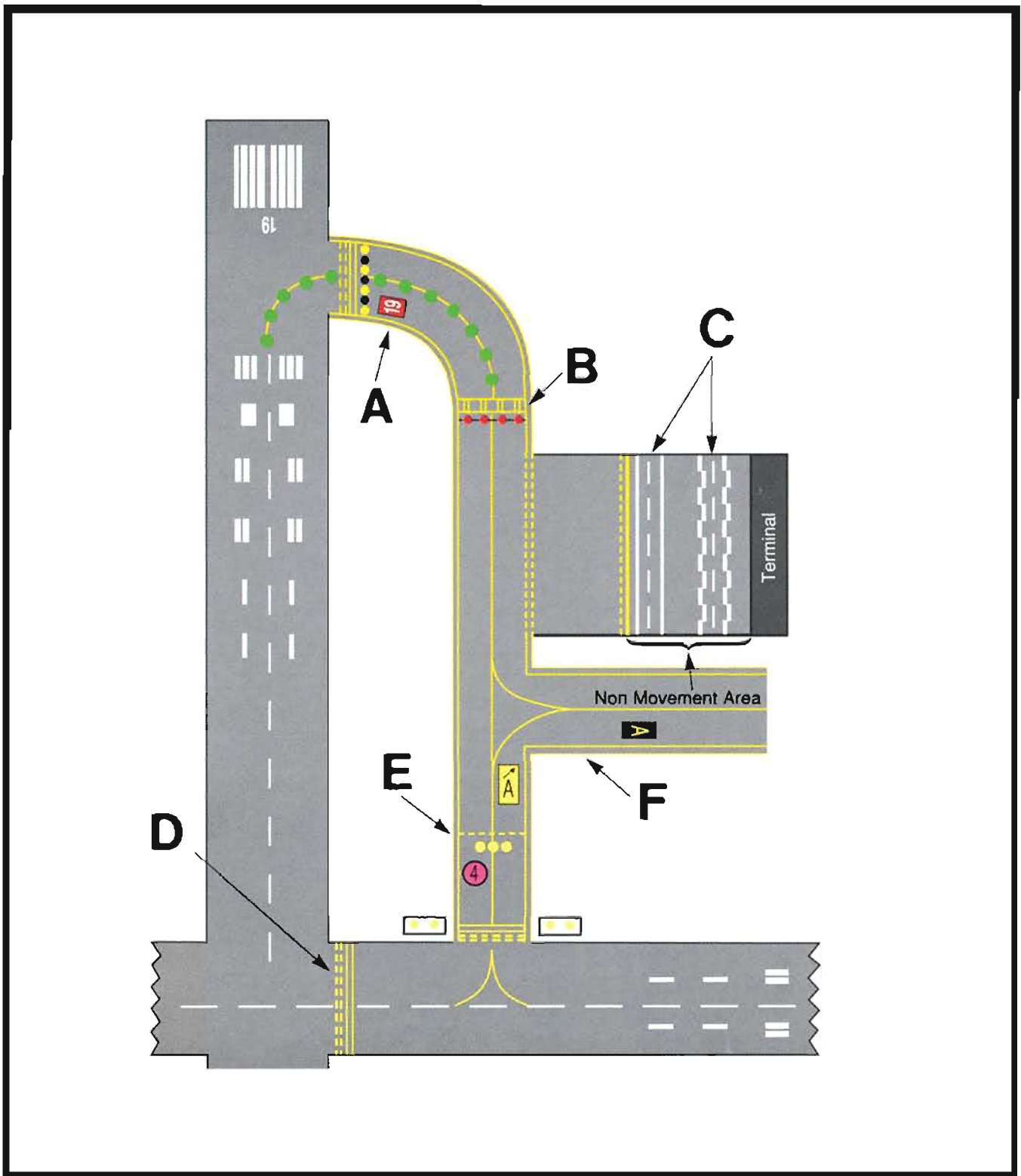
FIGURE 72.—Airport Markings.
