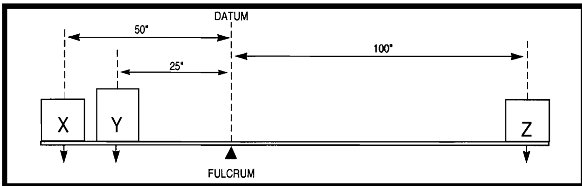
FIGURE 35.—Weight and Balance Diagram.
