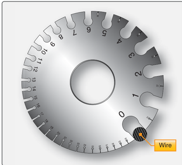
Figure 4-56. Wire gap gauge.
