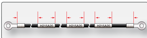
Figure 4-81. Spacing of printed identification marks.
