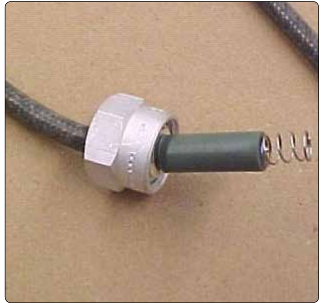
Figure 4-13. Ignition lead spark plug end.
