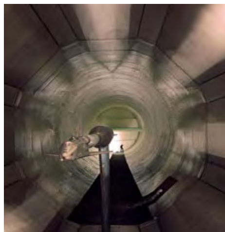
Model of the Space Shuttle in Langley's 16-Foot Transonic Tunnel.
