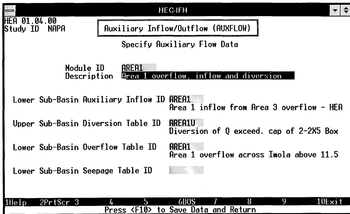
Figure 15. Auxiliary Flow Components for Interior Area 1 - HEA
