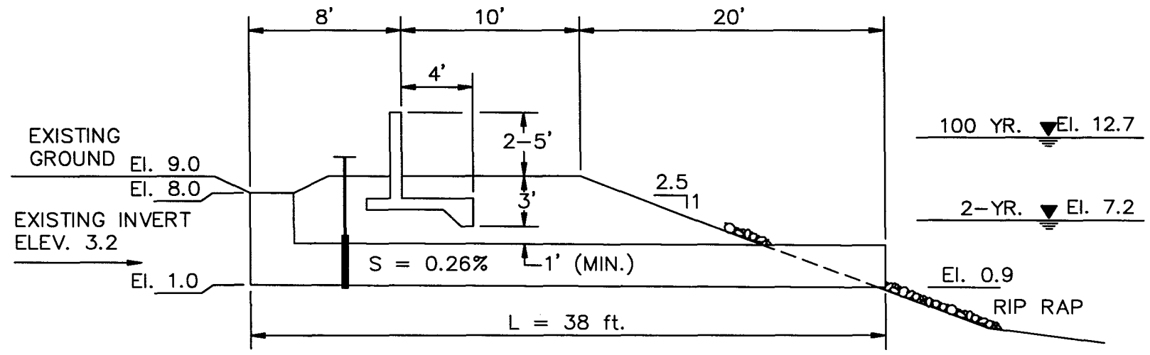
TYPICAL SET-BACK FLOOD WALL
