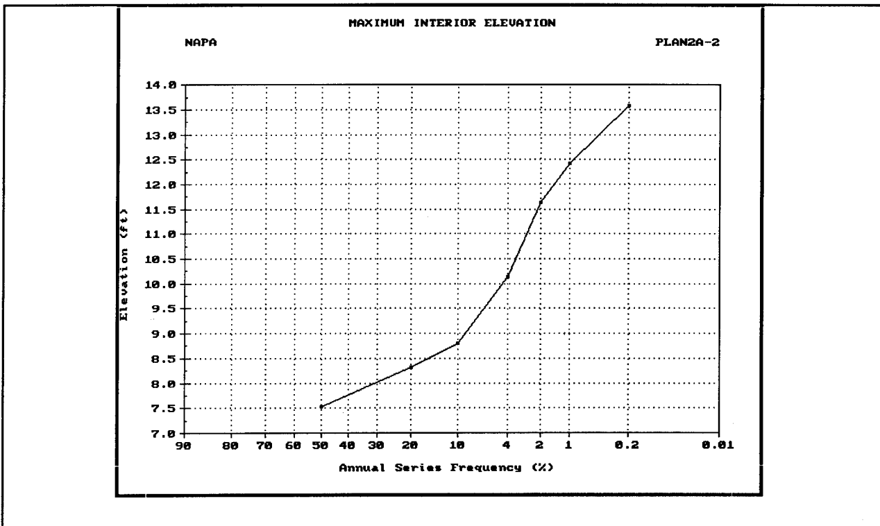
Figure 24. Interior Elevation-Frequency with Minimum Facility - Area 2A
