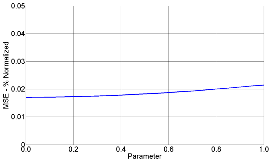
Figure 14. MSE for V2GHalf vs. V2GFull charging scenarios - PHEV-110
