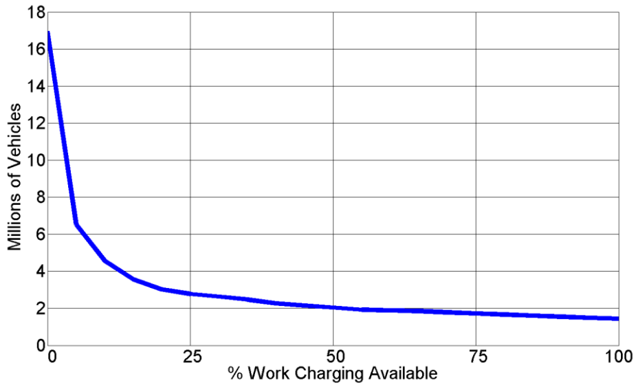
Figure 21. Population required to meet full additional imbalance; V2GHalf and V2GFull - PHEV-110
