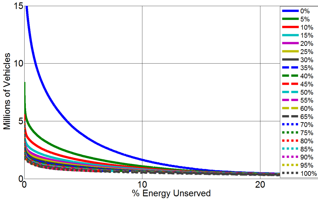
Figure 17. Unserved energy percentage for work charging availability, V2GHalf only - PHEV-110
