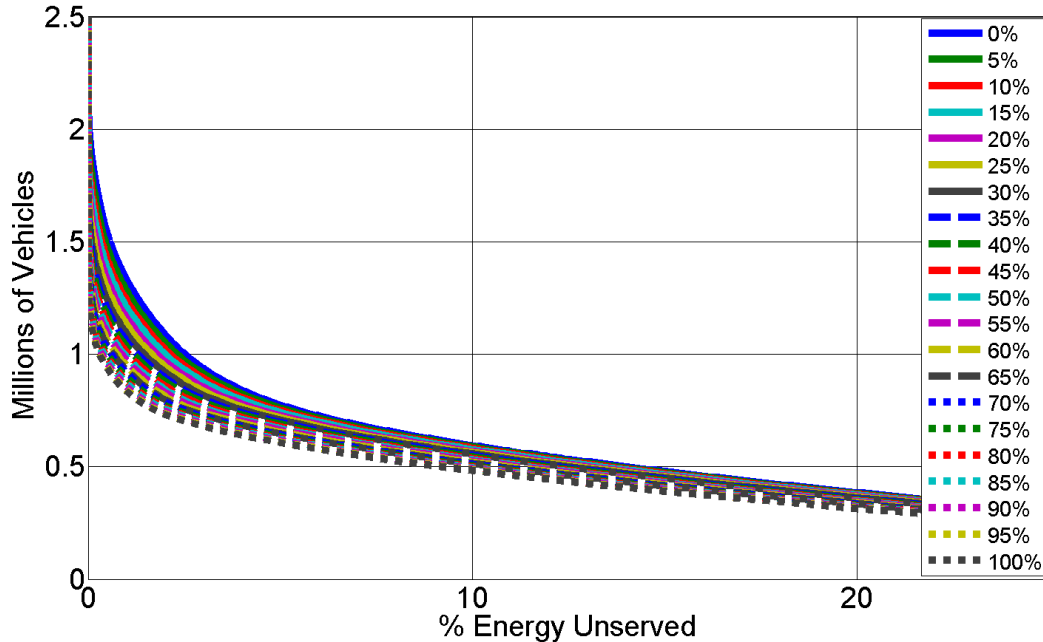
Figure 13. Unserved energy percentage for V2GHalf vs. V2GFull charging scenarios - PHEV-110 (note 0% means all vehicle perform V2Ghalf; 100% means all vehicle perform V2Gfull)
