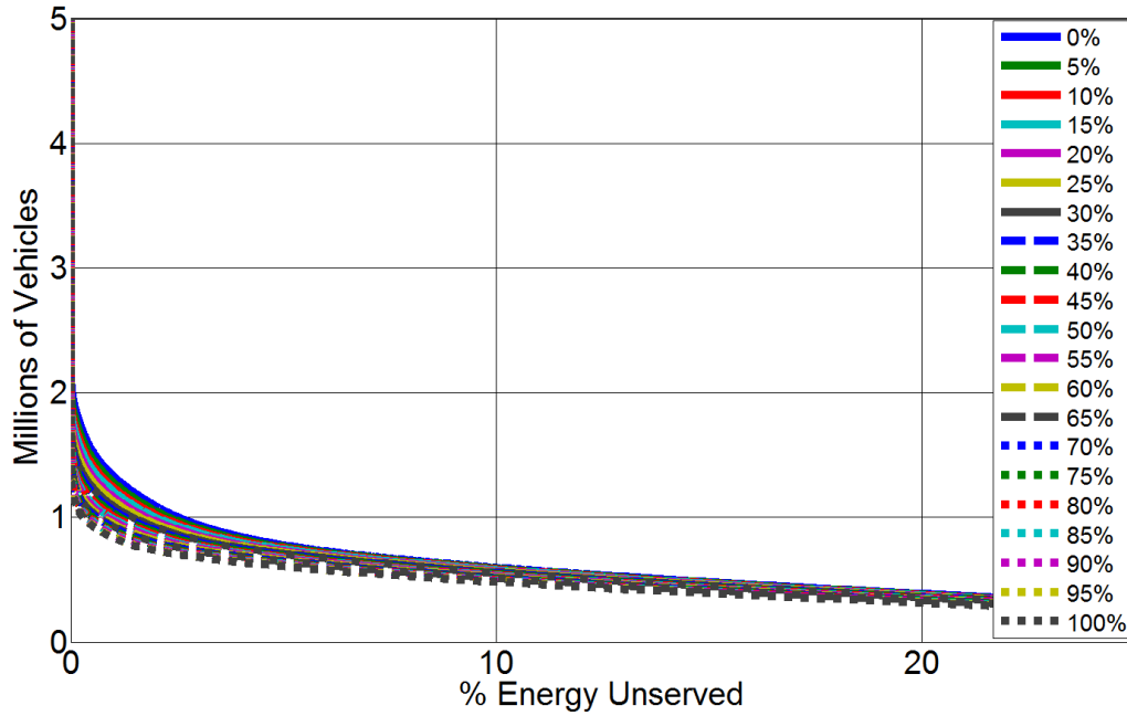
Figure A-1. Unserved energy percentage for V2GHalf vs. V2GFull Charging - PHEV-33
