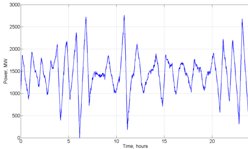
Figure 2. Single day of wind balancing data in NWPP
