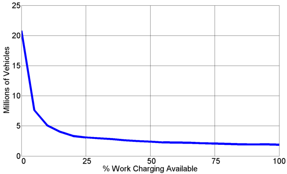
Figure 18. Population required to meet full additional imbalance - V2GHalf only - PHEV-110
