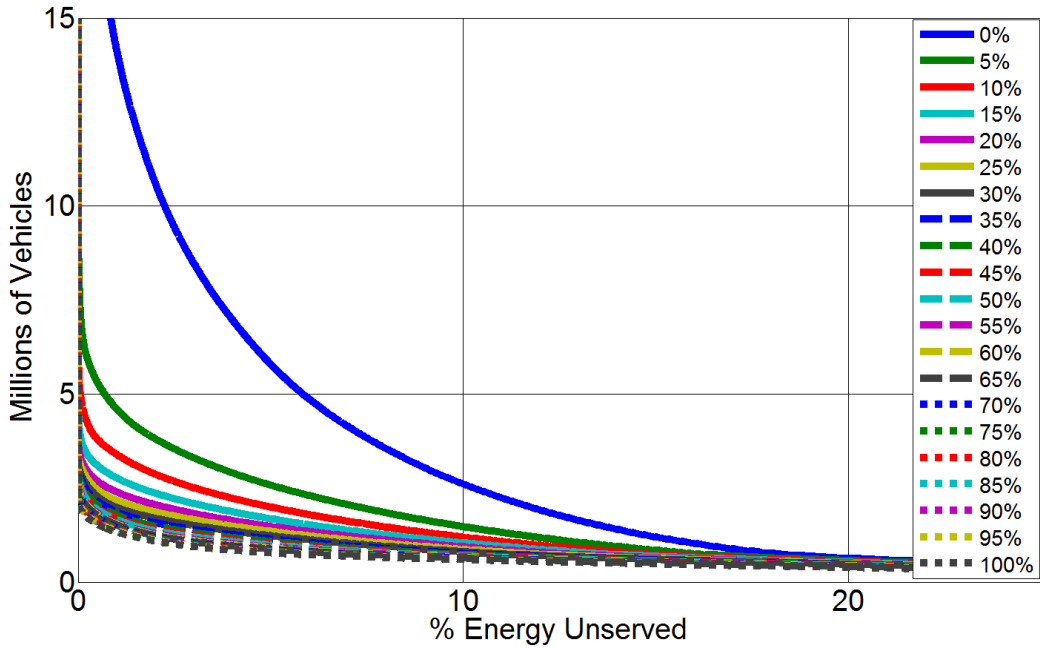
Figure A-5. Unserved energy percentage for work charging availability - V2GHalf only - PHEV-33
