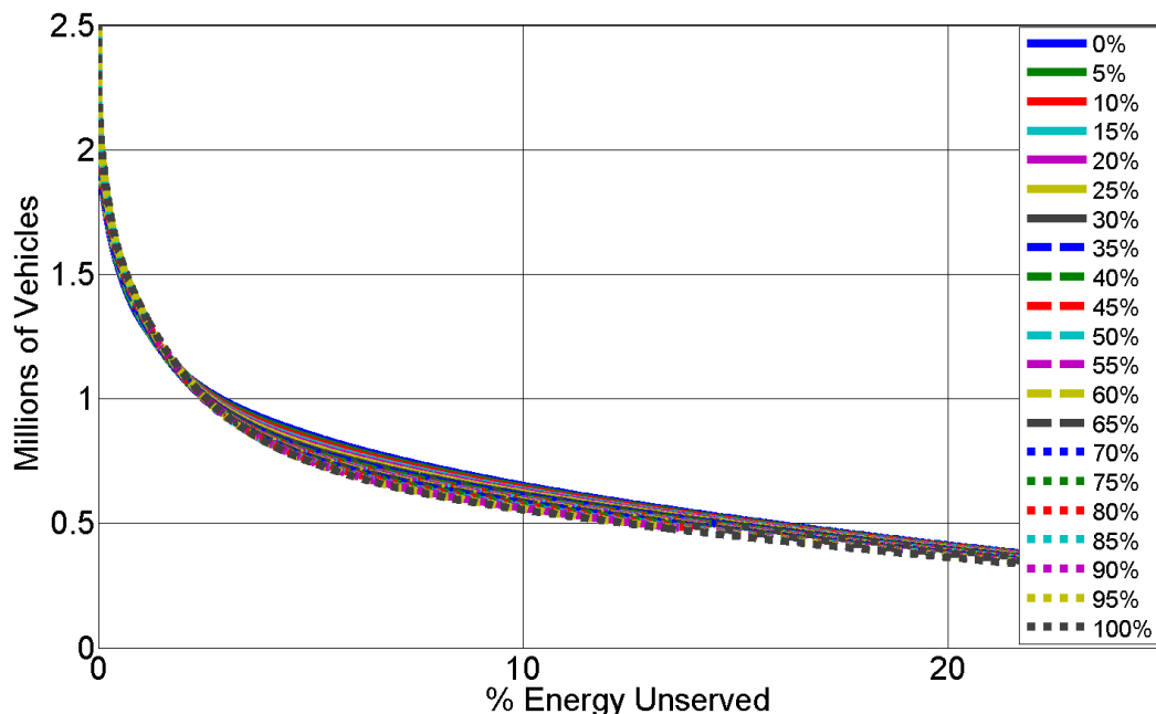
Figure 15. Unserved energy percentage for home Level 2 charging availability - V2GHalf only - PHEV-33 (note 0% means all vehicle charge at Level 1; 100% means all vehicle charge at Level 2)
