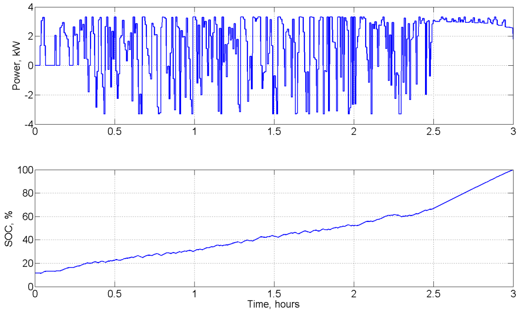
Figure 7. Vehicle-to-grid-full (V2GFull) charging example
