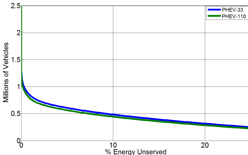
Figure 12. Unserved energy percentage for ideal V2GFull charging scenarios
