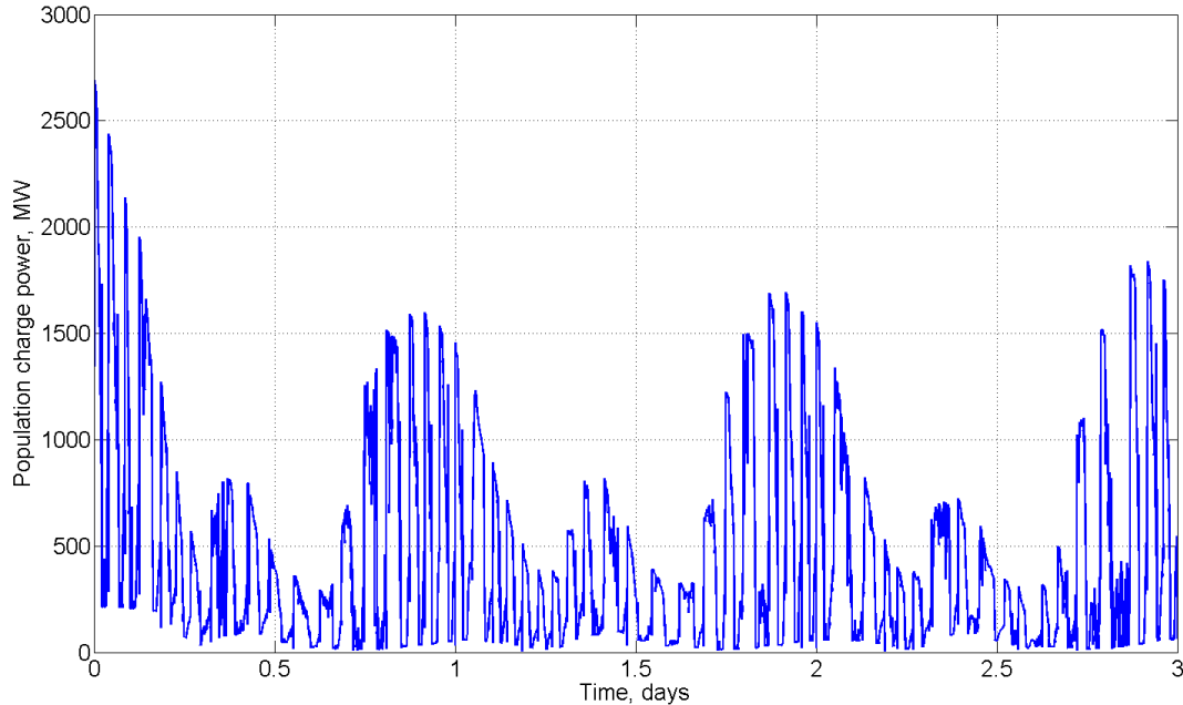
Figure 5. Population charge rate over three-day period
