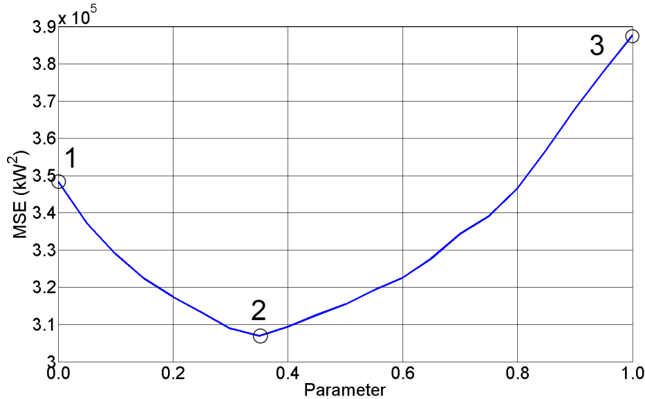
Figure 9. Example MSE plot for 1 million vehicles
