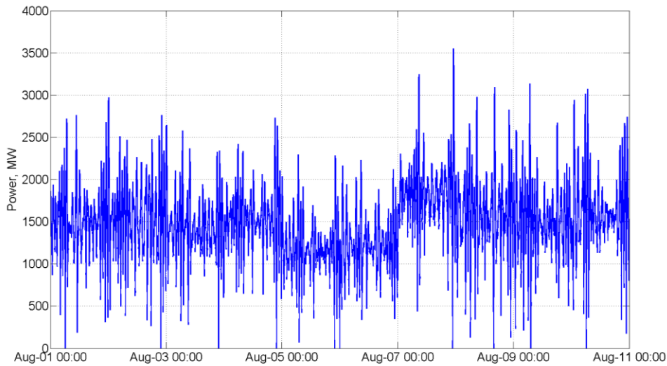
Figure 1. Balancing signal for 14.4 GW of wind generation in NWPP
