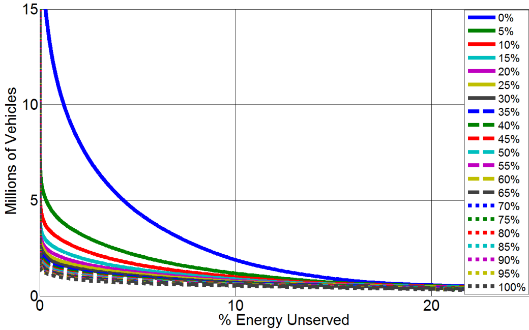
Figure A-7. Unserved energy percentage for work charging availability - V2GHalf and V2GFull - PHEV-33
