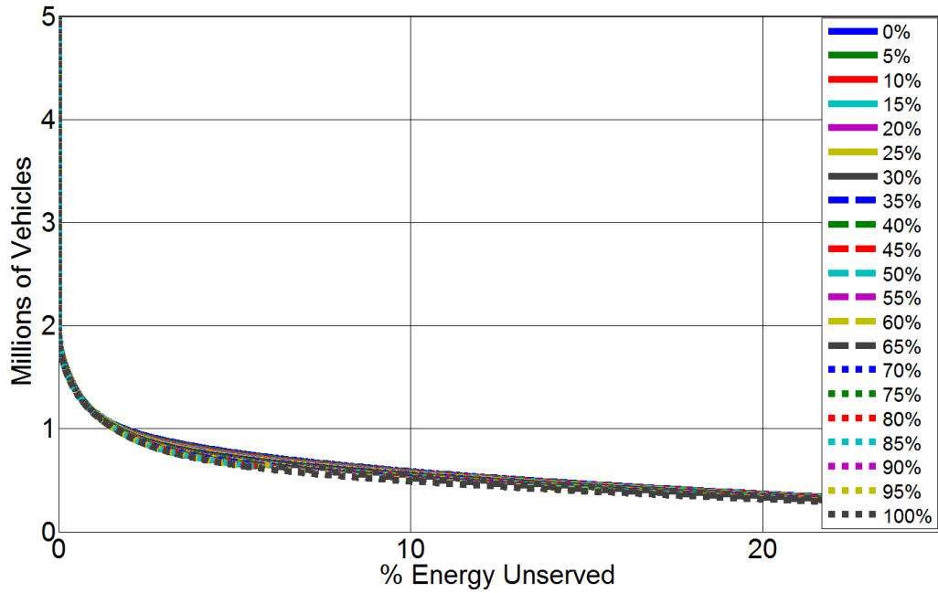
Figure A-3. Unserved energy percentage for home 240-Volt charging availability - V2GHalf only - PHEV-110
