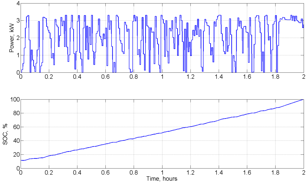
Figure 6. Vehicle-to-grid-half (V2GHalf) charging example
