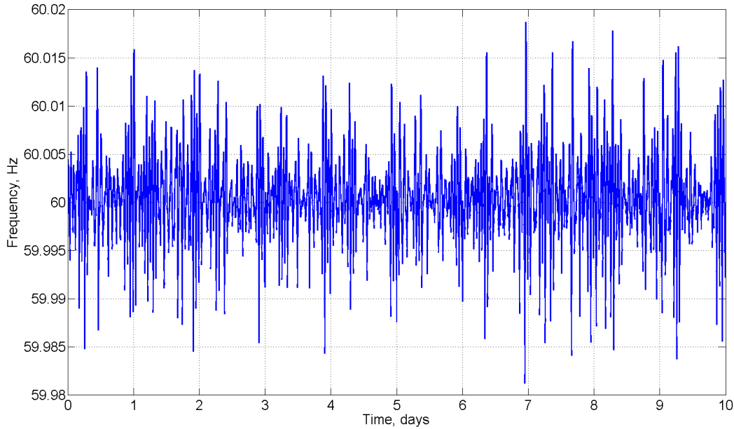
Figure 3. Grid frequency from balancing signal
