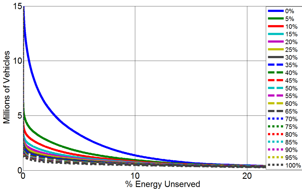
Figure 20. Percentage of Unserved energy for work charging availability - V2GHalf and V2GFull - PHEV-110
