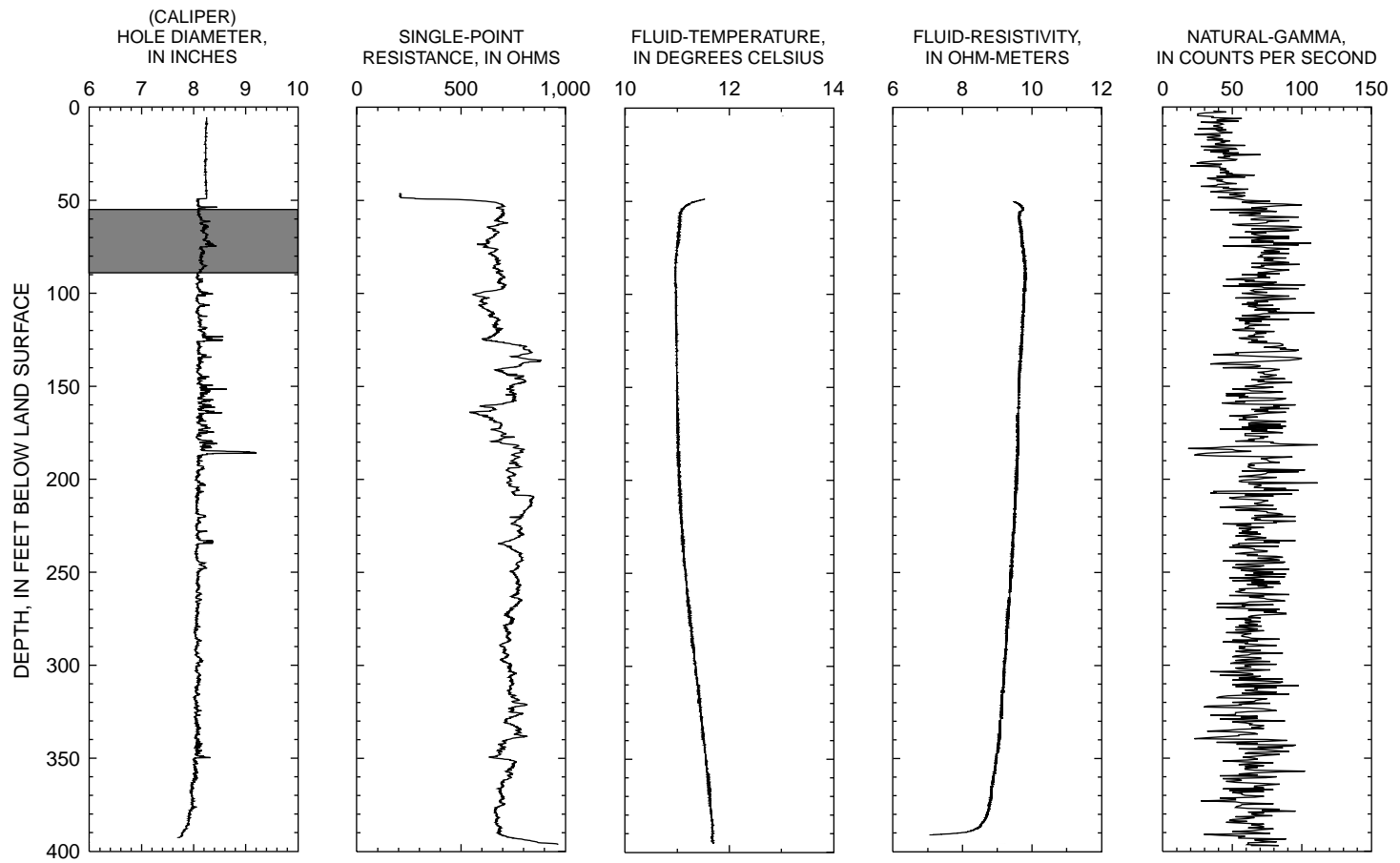
Figure 4. Borehole-geophysical logs for borehole CL-AD-175 (HN-1D), Keystone Sanitation Superfund Site. Shaded area on caliper log shows water-producing zone.
