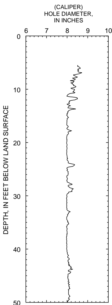
Figure 2. Borehole-geophysical log for borehole CL-AD-173 (HN-1S), Keystone Sanitation Superfund Site.
