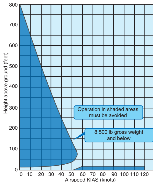
Figure 10-10. Height/velocity chart.
