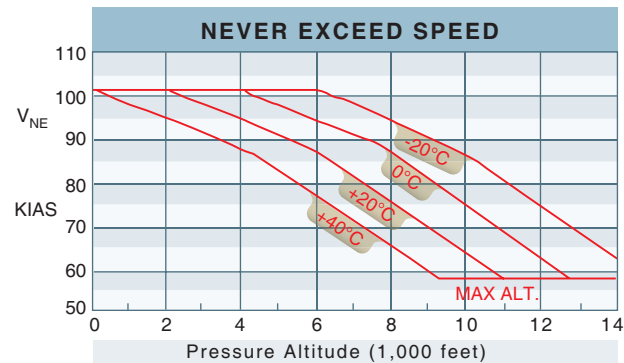
Figure 5-6. Various V_{NE} placards.
