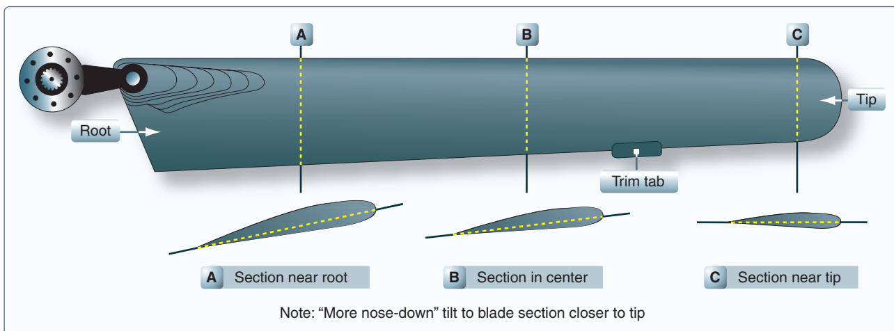
Figure 2-12. Blade twist.
