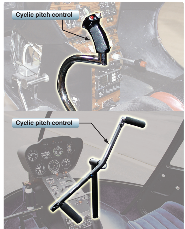
Figure 3-4. The cyclic pitch control may be mounted vertically between the pilot's knees or on a teetering bar from a single cyclic located in the center of the helicopter. The cyclic can pivot in all directions.
