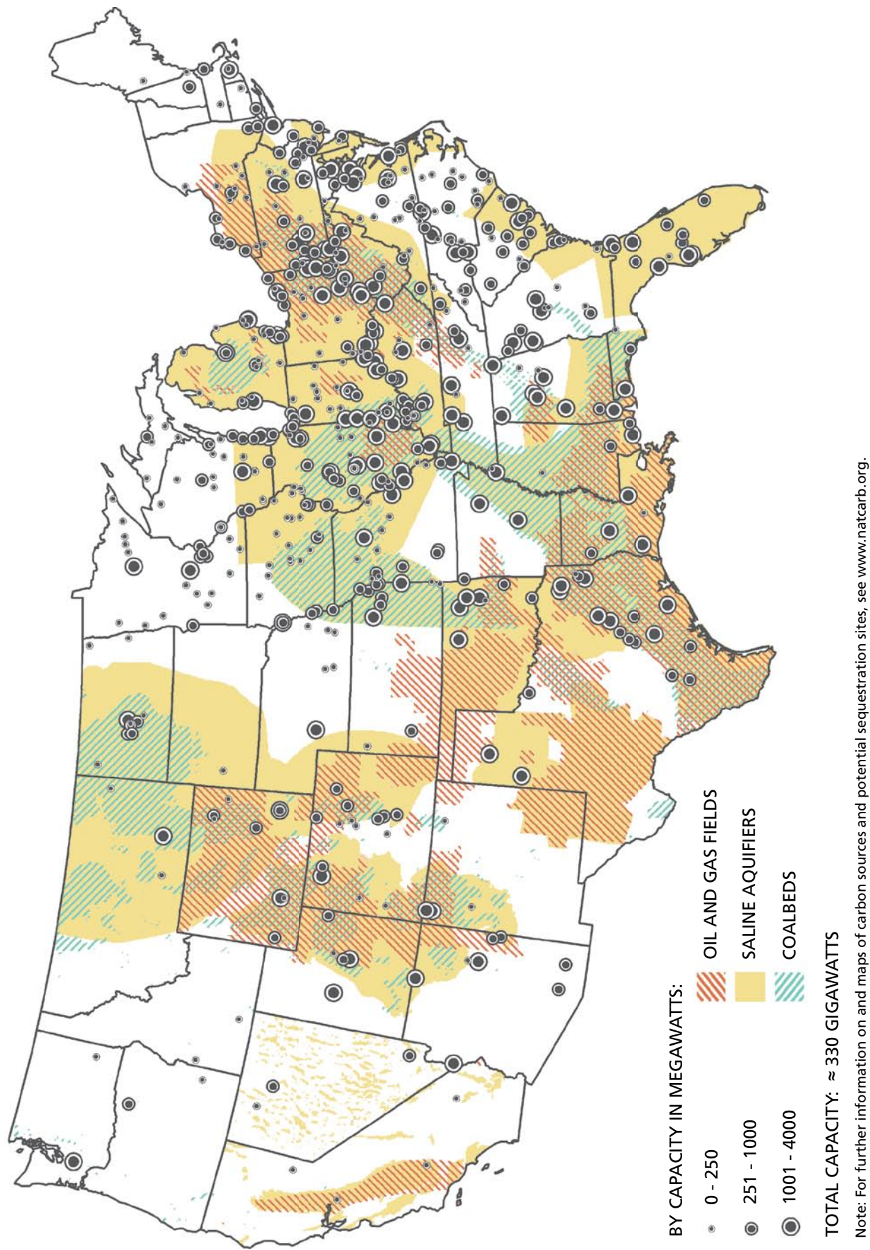
FIGURE 5-3. U.S. Coal-Fired Power Plants (2000) and Potential Sequestration Sites
