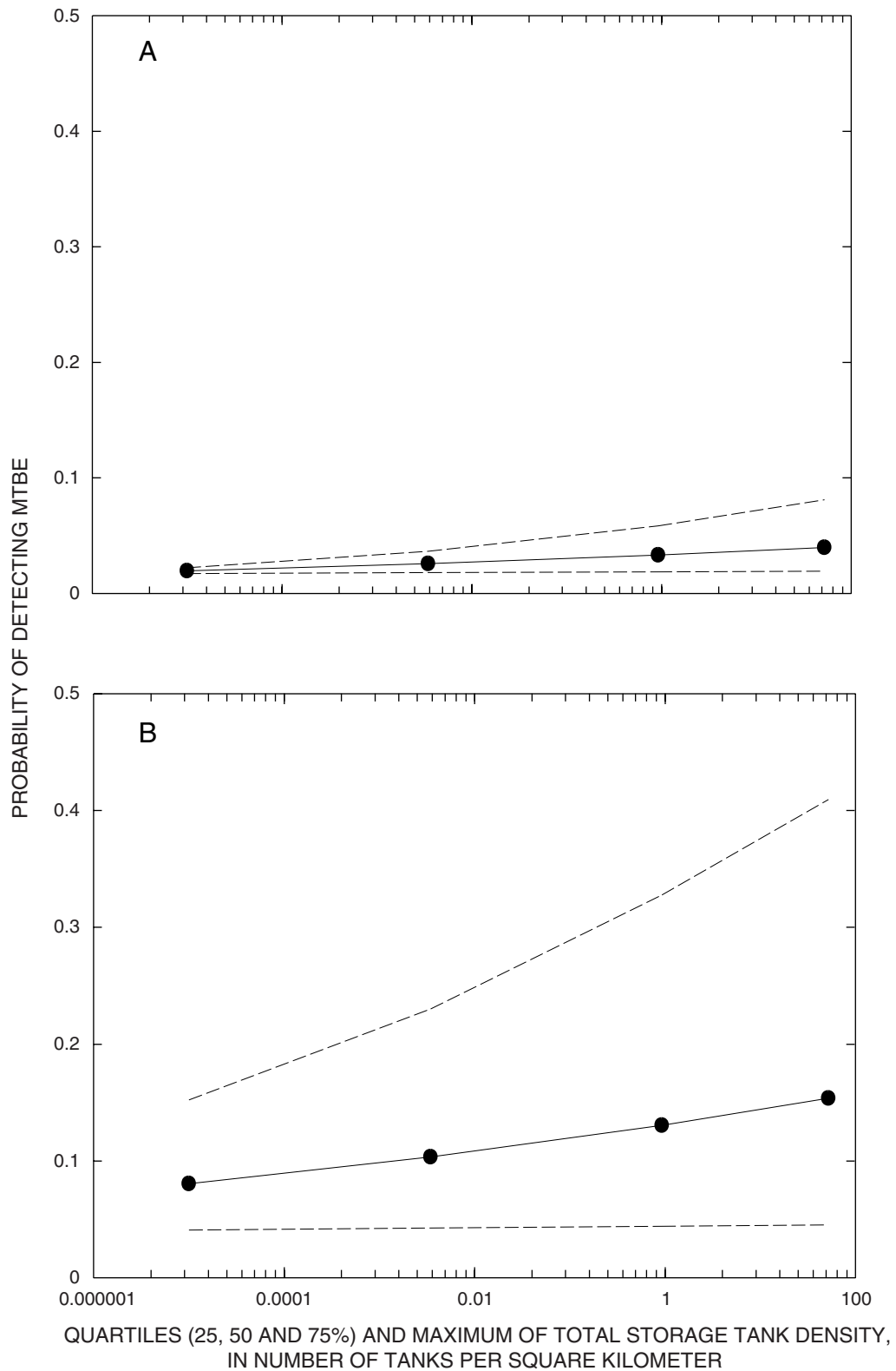
Figure 2. Estimated probabilities of detecting MTBE (methyl tert -butyl ether) in (A) areas of little MTBE use and (B) areas where MTBE is used in the Reformulated (RFG) or Oxygenated (OXY) gasoline programs with high soil erodability according to the logistic model described by equation 1.
