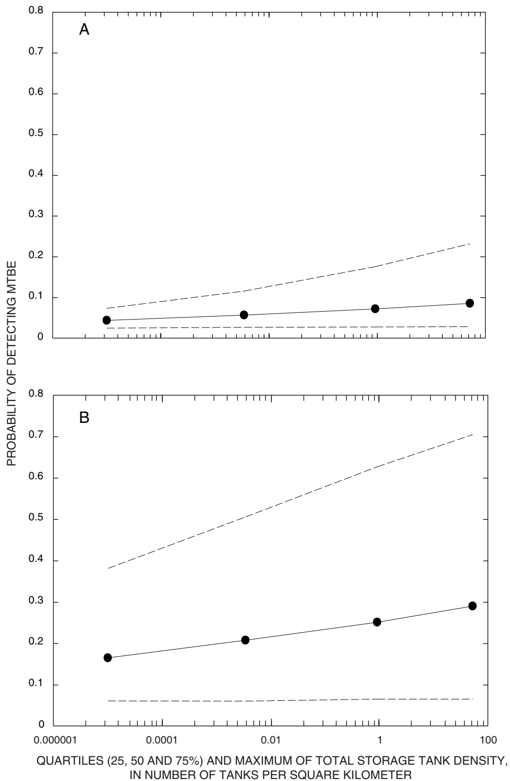
Figure 3. Estimated probabilities of detecting MTBE (methyl tert -butyl ether) in (A) areas of little MTBE use and (B) areas where MTBE is used in the Reformulated (RFG) or Oxygenated (OXY) gasoline programs with low soil erodability according to the logistic model described by equation 1.
