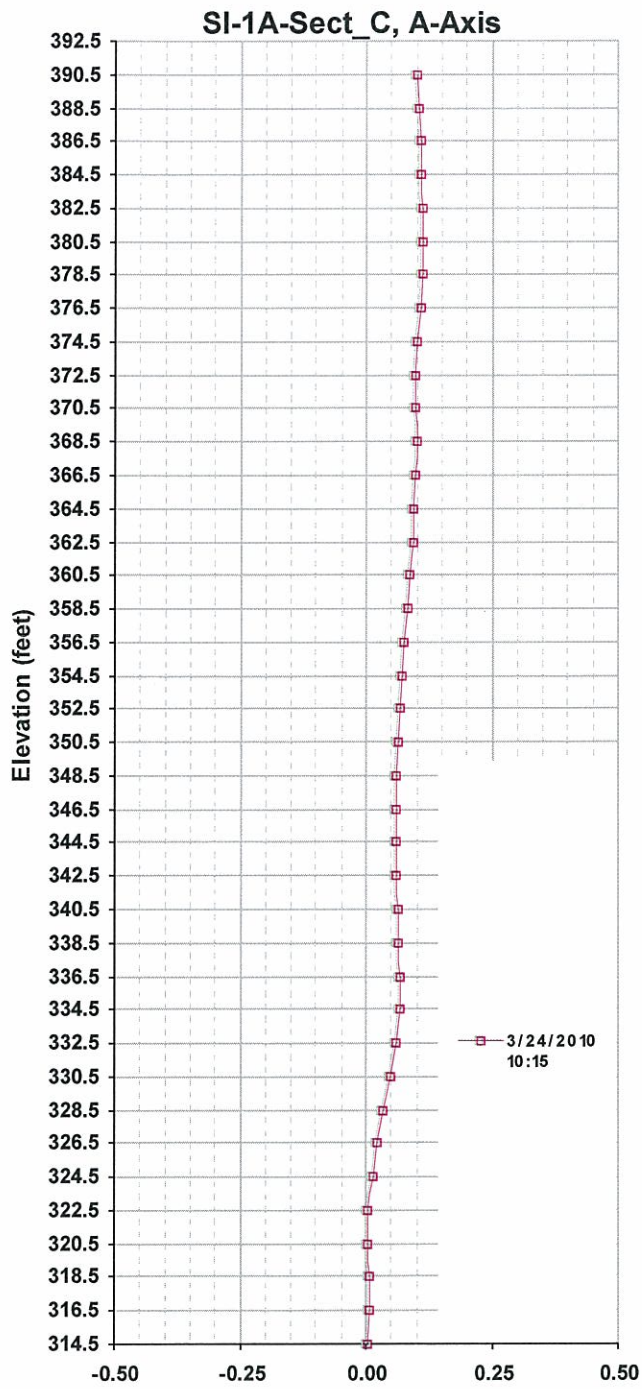
Cumulative Displacement (in) from 2/22/2010
