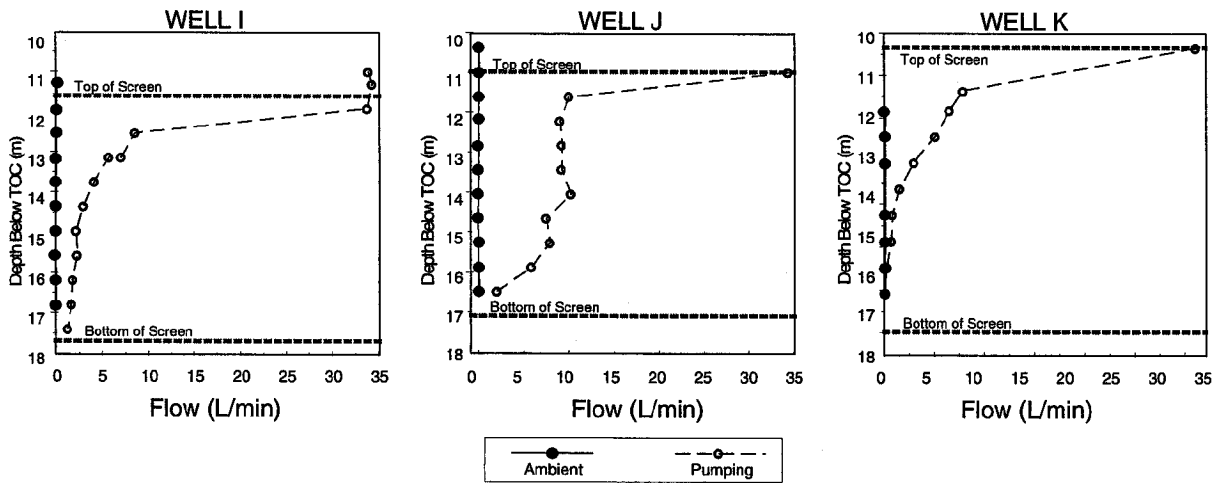
Figure VII-5. Ambient and induced flow distributions for wells I, J, and K at the Gilson Road site.
