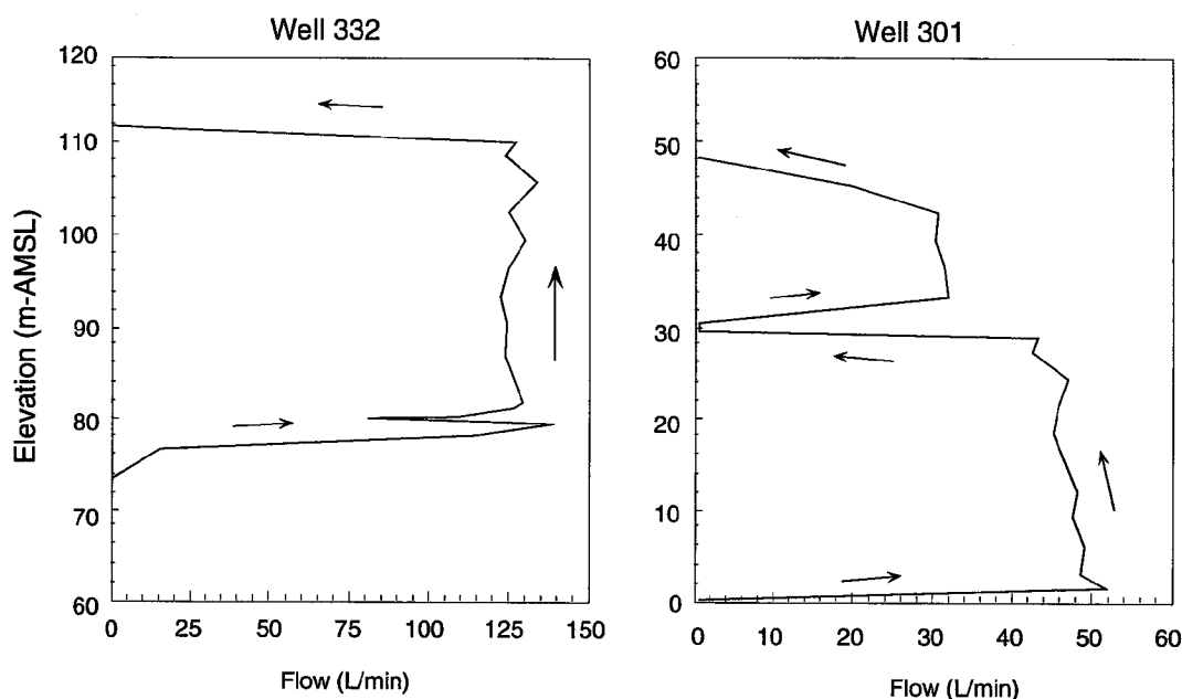
Figure VII-7. Substantial ambient flow moving from one stratum to another as detected by an impeller flowmeter. The flow is moving under a dam, the base of which is at an elevation of about 140 m AMSL. Flowmeter data were used to help select a geologic model for explaining the large leakage of water low in dissolved oxygen that was observed below the dam.
