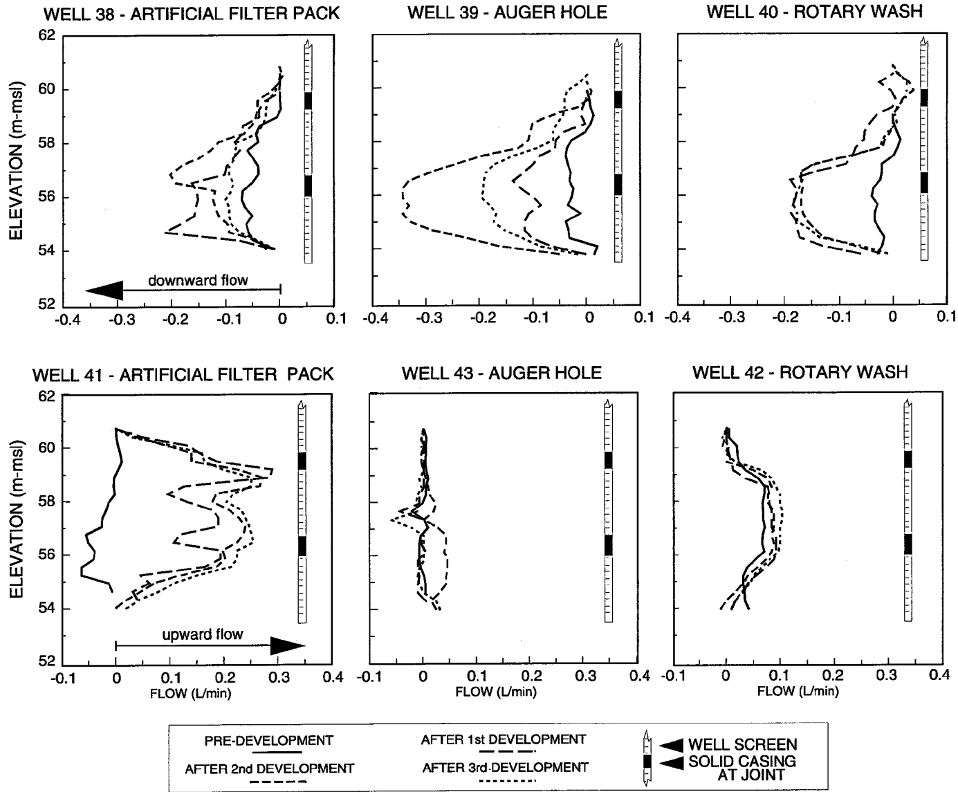
Figure V-4. Ambient flow profiles after successive well development.
