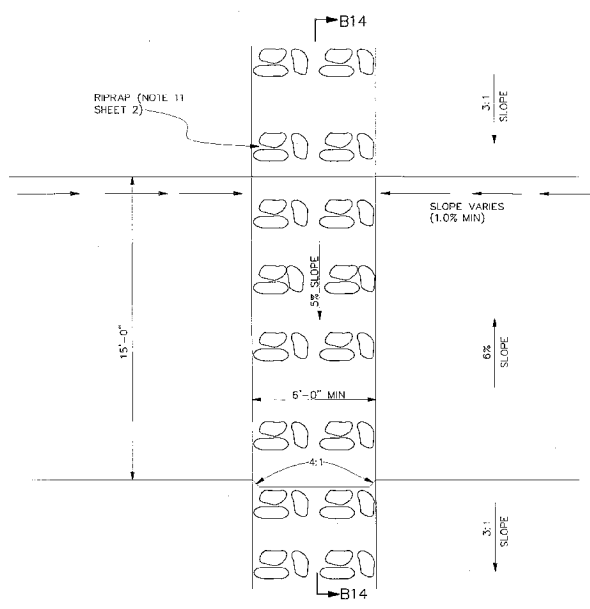
RIPRAP DOWN DRAIN COVER OPTION 1
