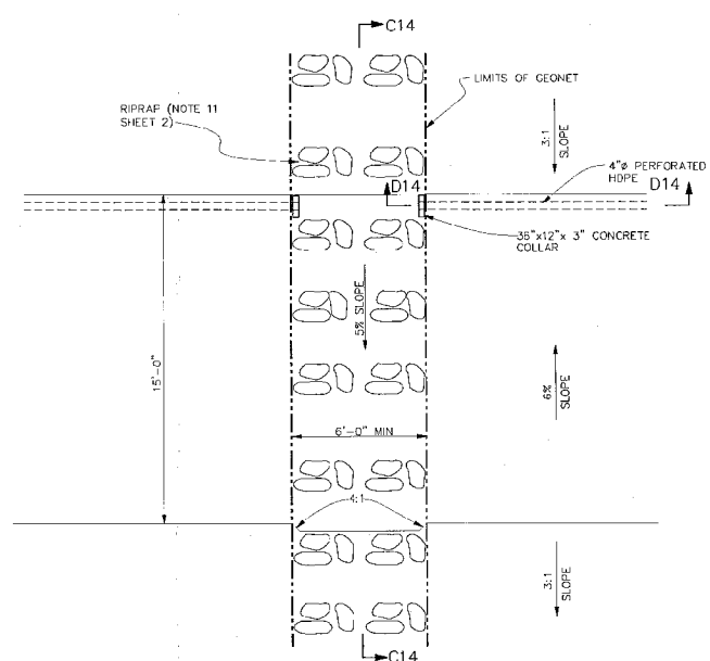
RIPRAP DOWN DRAIN COVER OPTION 2
