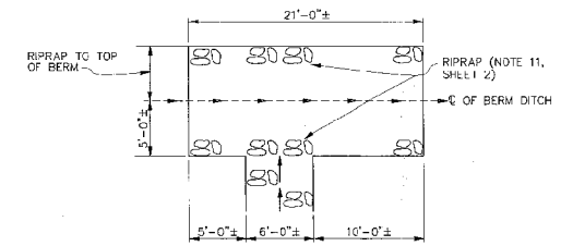
DETAIL F14 3/16" = 1'-0"
