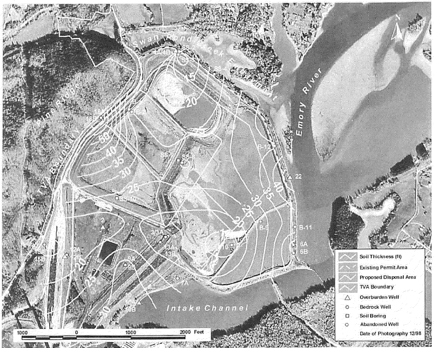
Figure 2-5. Alluvium-Residuum Thickness Map
