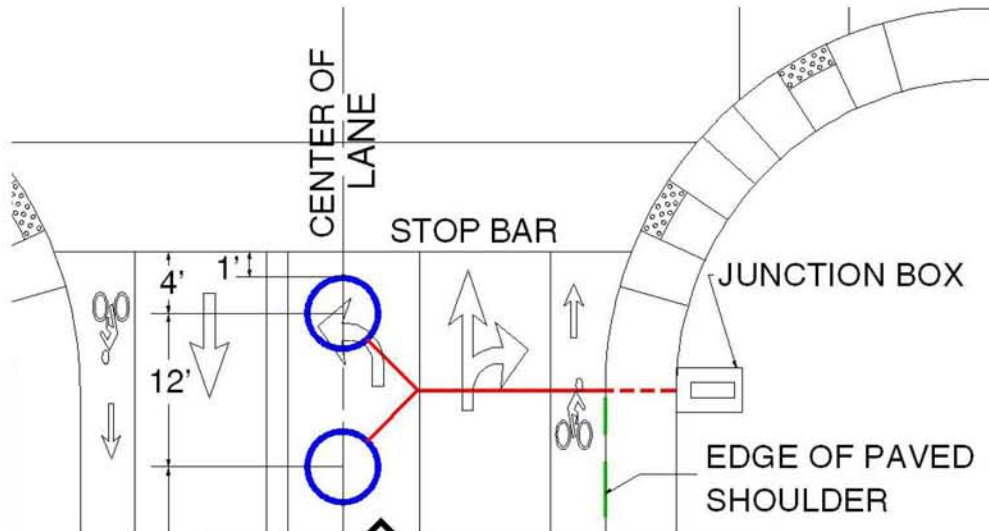
(a) Schematic design of loop detector design
