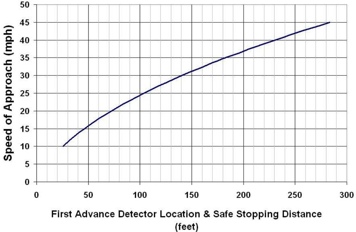
Figure 4-20 Detector location for multiple detector technique (level approach)
