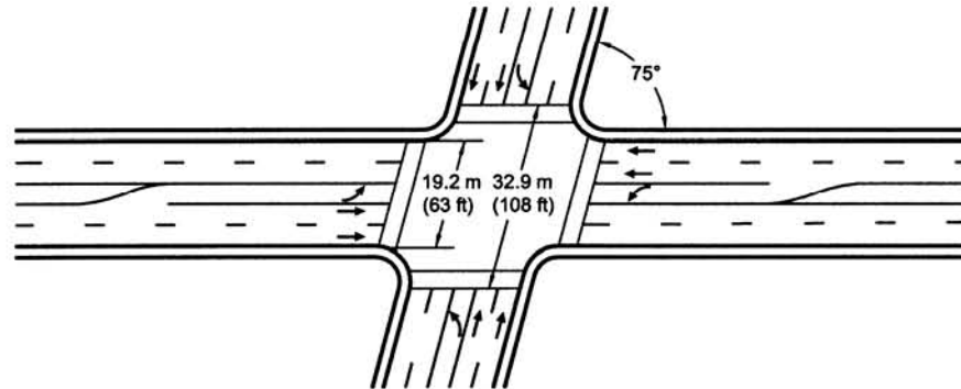
(b) Intersection skew at 75 degrees
