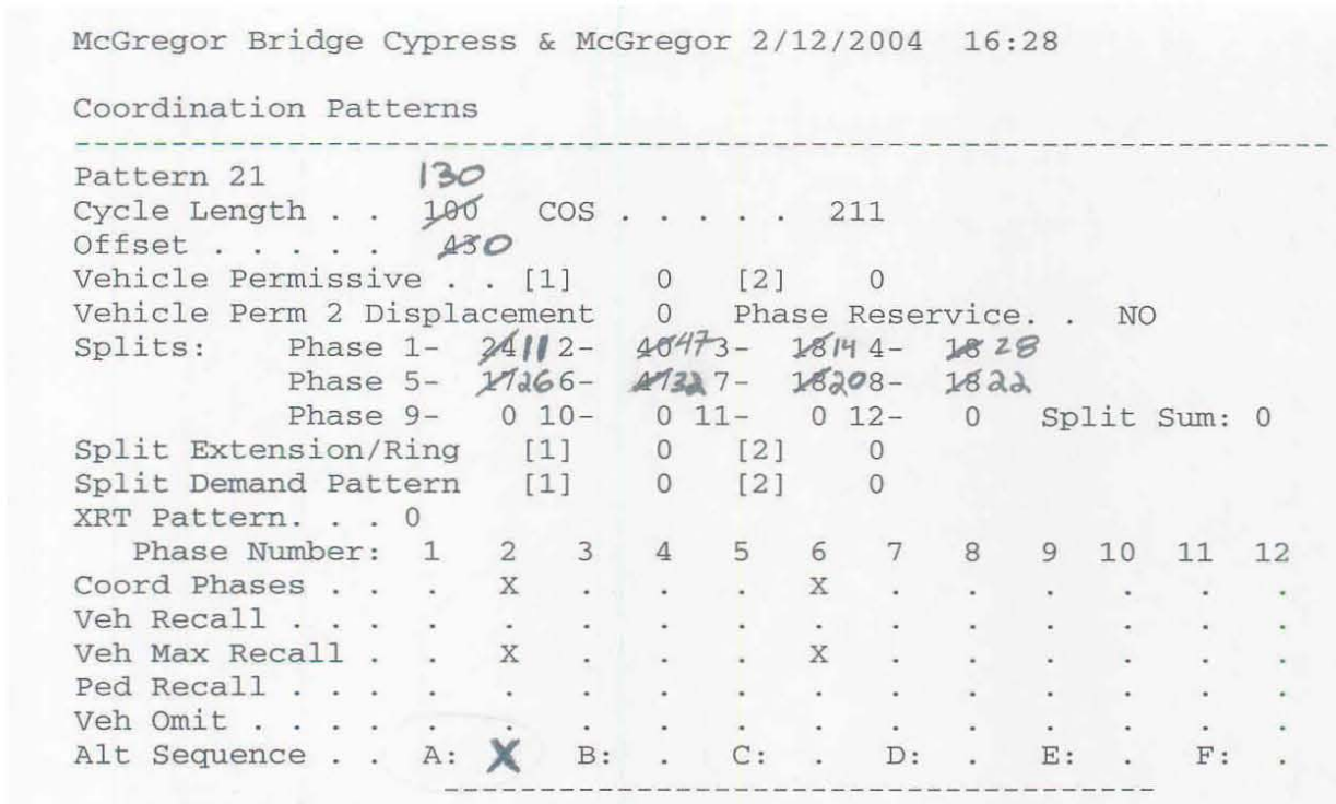
Figure 7-14 Controller Markup
