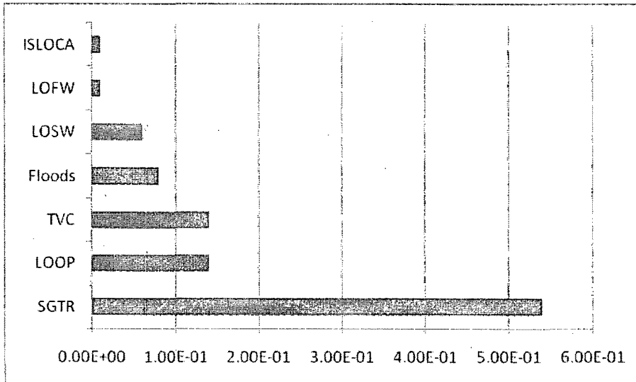
Figure E.2-4 Individual Initiator Contribution to LERF
