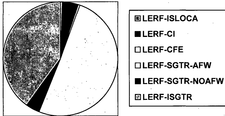
Figure E.2-9 LERF Contributors by Release Category
