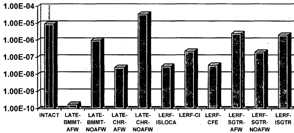
Figure E.2-7 Results for Detailed Release Categories
