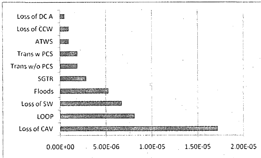
Figure E.2-2 Individual Initiator Contribution to CDF
