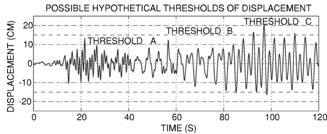
Figure 12. Hypothetical thresholds of displacements shown to demonstrate how GPS data can be configured to provide alarms at different amplitudes. Decision makers can use this information in various ways. (This particular record is for demonstration only. It is 20 times amplified from the double-integrated acceleration record of CH21 [vertical at side-span] of Vincent Thomas Bridge in Los Angeles Harbor [1996 M=6.7 Northridge earthquake]—a California Division of Mines and Geology [CDMG] record.)
