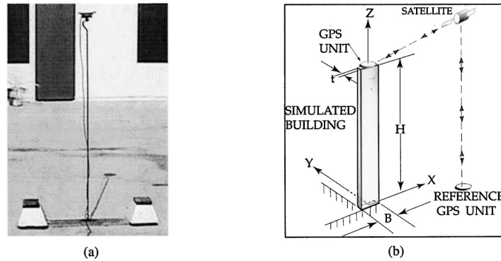
Figure 1. Photo (a) and schematic (b) of test set-up to simulate using GPS for dynamic monitoring of tall buildings.
