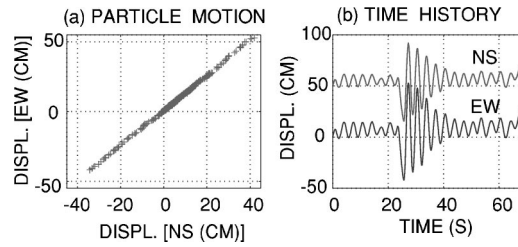
Figure 2. Particle motion and time-history of relative displacements (NS and EW components) of simulated test specimen.
