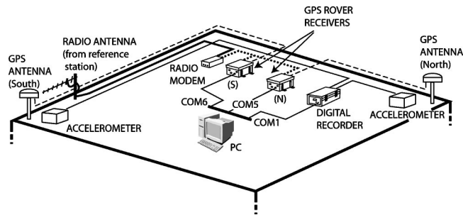
Figure 6. Details of the connections between GPS, radio modems, accelerometers, and the PC.
