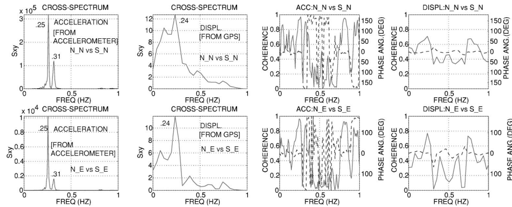
Figure 11. Cross-spectra ( S_{xy} ) and associated coherency and phase angle plots of horizontal, parallel accelerations and displacements.
