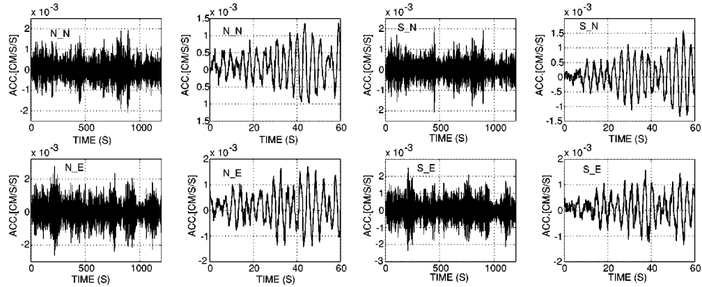
Figure 9. Remotely triggered and recorded accelerations at N (north) and S (south) locations. The figure shows pairs of 1200-second-long (and 60-second window from the same) record.
