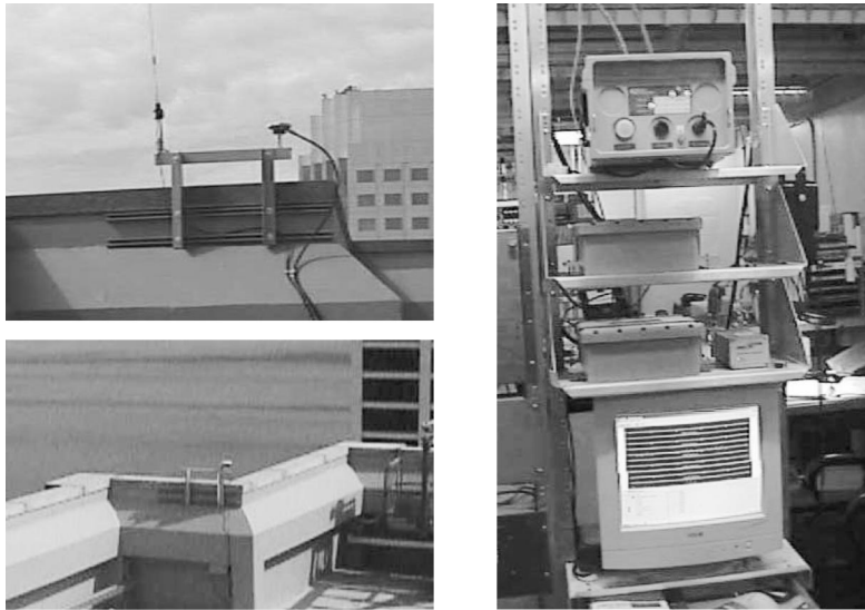
Figure 7. GPS and radio modem antennas at the diagonal corners of the building and the PC receiving streams of GPS and accelerometer data in real time. Shown above the PC are the accelerometer recorder and the GPS Rover units.
