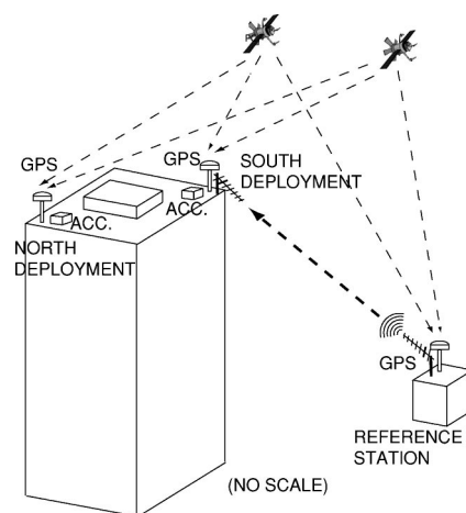
Figure 5. General schematic of the GPS deployment in San Francisco, CA.
