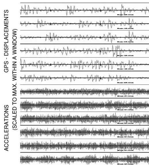
Figure 8. A window of data streaming in real time, captured from the PC monitor.
