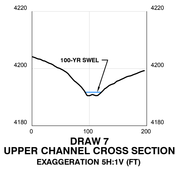
DRAW 7 UPPER CHANNEL CROSS SECTION EXAGGERATION 5H:1V (FT)
