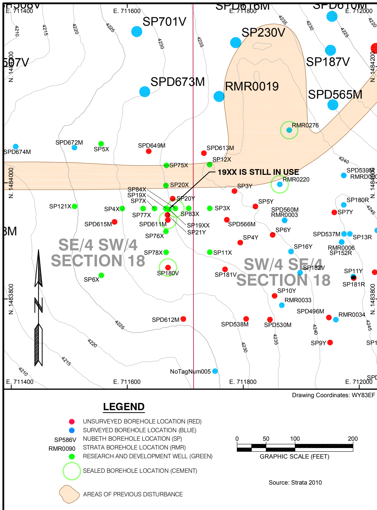
Figure 2. Phase I Research and Development Area
