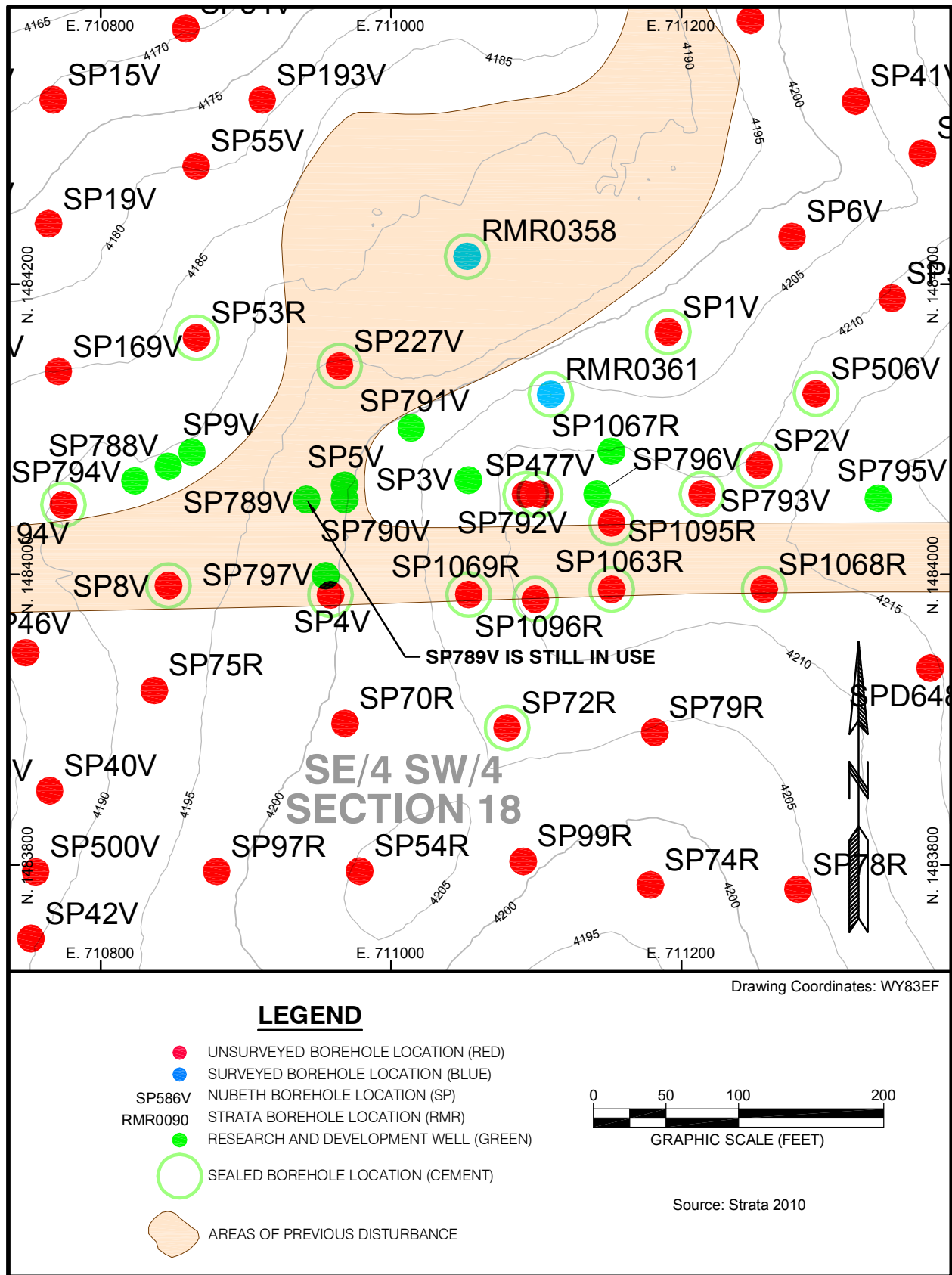
Figure 1. Hydrologic Test Area
