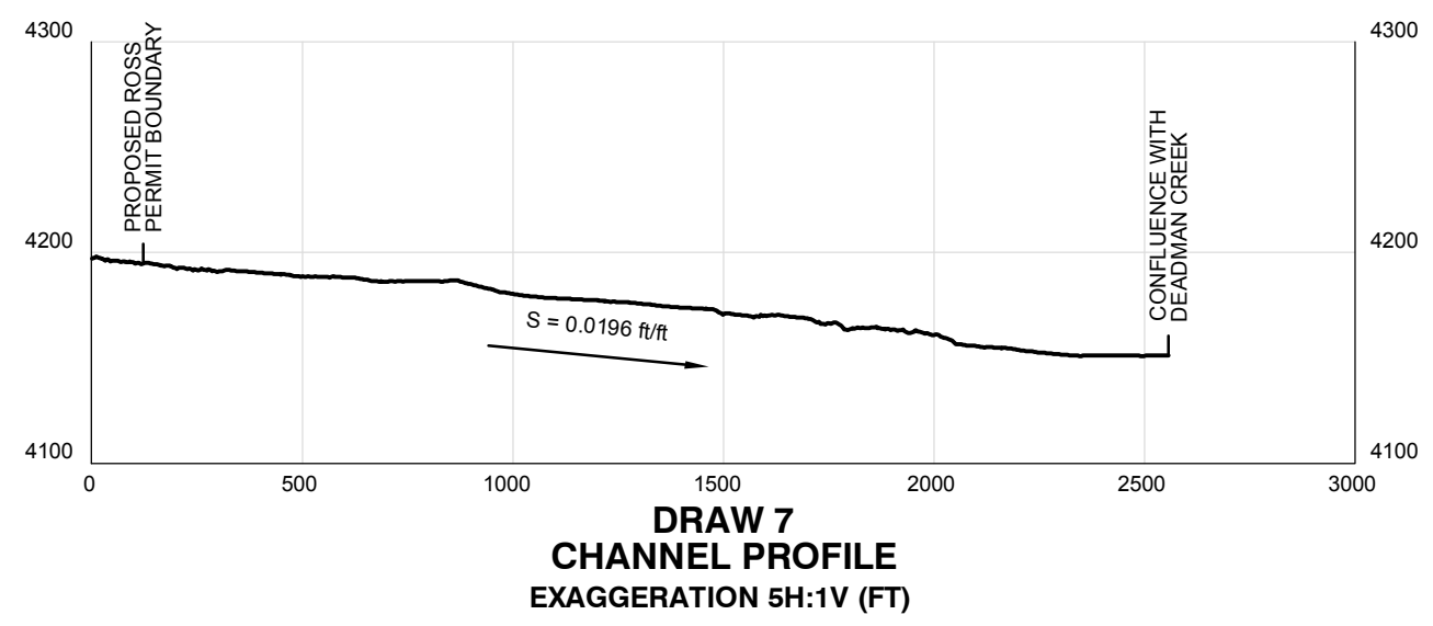
DRAW 7 CHANNEL PROFILE EXAGGERATION 5H:1V (FT)
