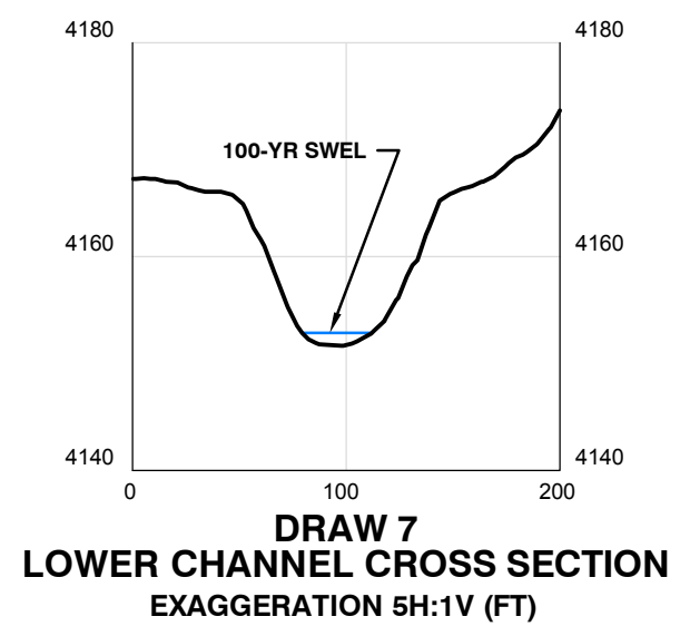
DRAW 7 LOWER CHANNEL CROSS SECTION EXAGGERATION 5H:1V (FT)
