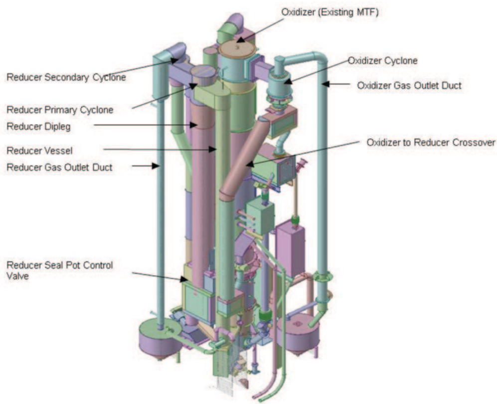
Figure 3: General Arrangement of 3\text{-MW}_{\text{th}} Prototype Test Facility
